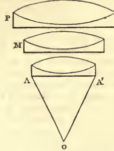
Section of the English achromatic combination.
