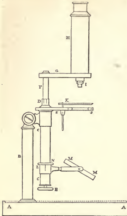
Superior Compound Microscope.
