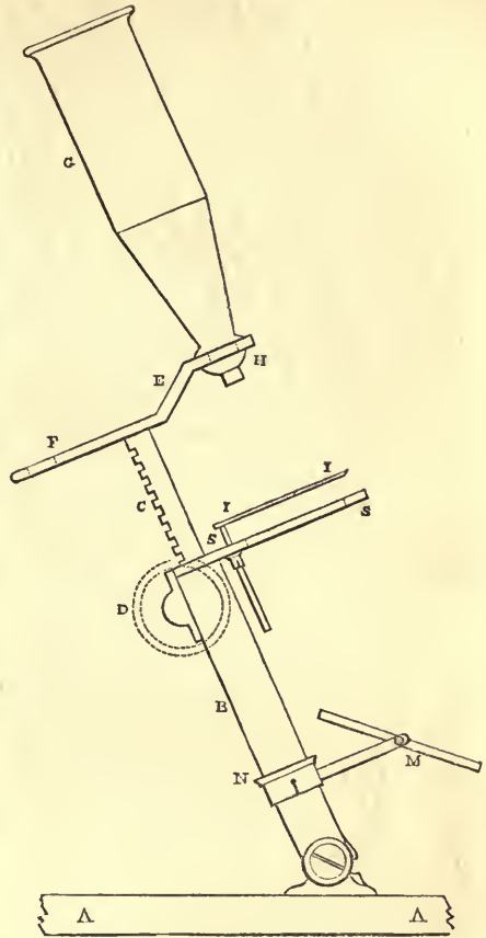
Elevation of ordinary compound or simple microscope.
