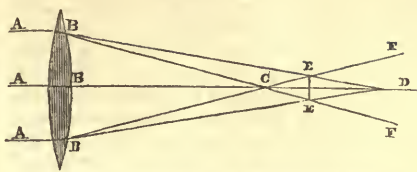
Diagram illustrative of chromatic aberration.
