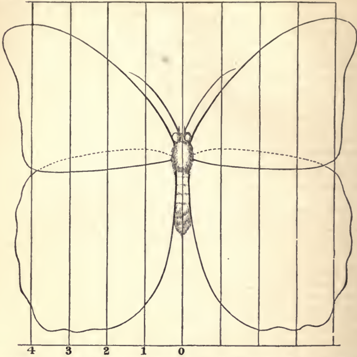
Distances of parallels from the axis of the body in 0.4 of an inch. ( Morpho autumedon .)
