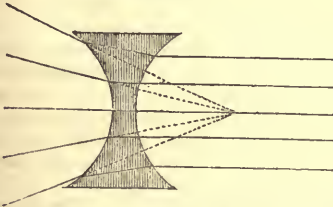
Parallel rays made to diverge as from the principal focus, and rays converging to that focus rendered parallel.
