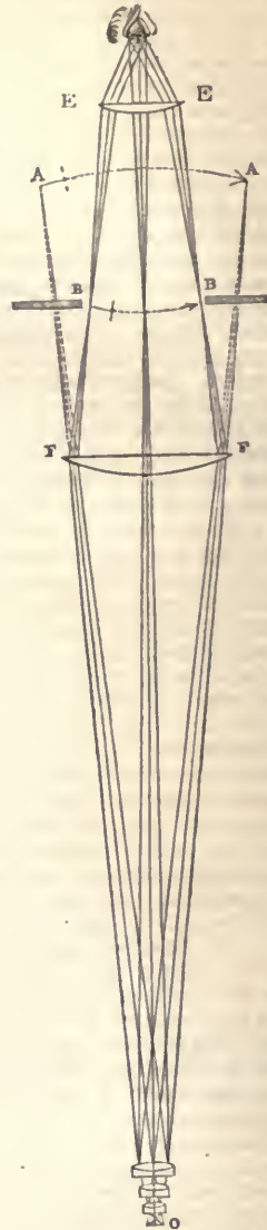
Section of Compound Microscope, with field-glass introduced.
