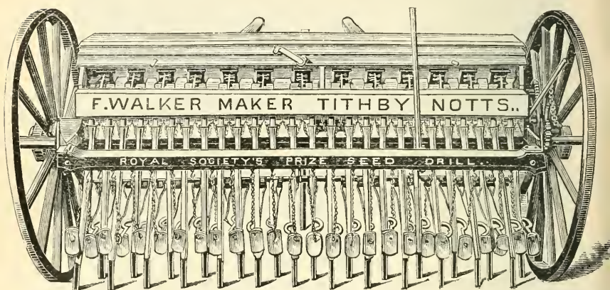
FIG. 4.—F. Walker & Sons' First Prize Coulter and Broadcast Drill for Grass and Clover, Class II.
