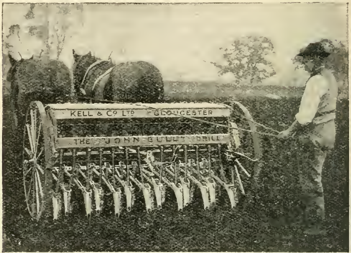
FIG. 3.—Kell & Co's H.C. "John Bull" 13-row Corn and Seed Drill, Class I.
