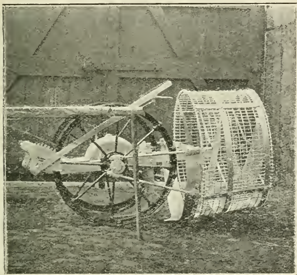
FIG. 3.—Potato Digger.
