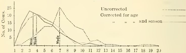
FIG. 8.—INDIVIDUAL VARIATION (RANGE) IN QUARTS. In 110 Cows during 6 years.
