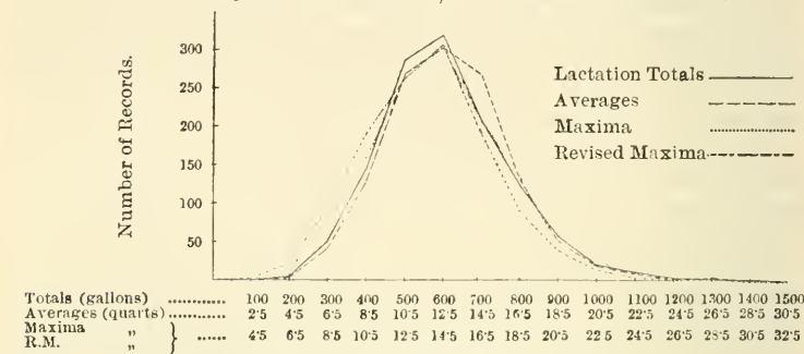
FIG. 1.—FREQUENCY CURVES: 1,233 NORMAL LACTATIONS.
