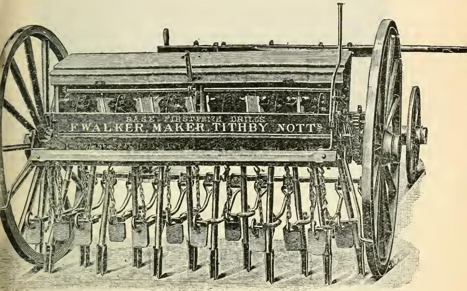
FIG. 2.—F. Walker & Sons' Second Prize 12-row Corn and Seed Drill, Class I.
