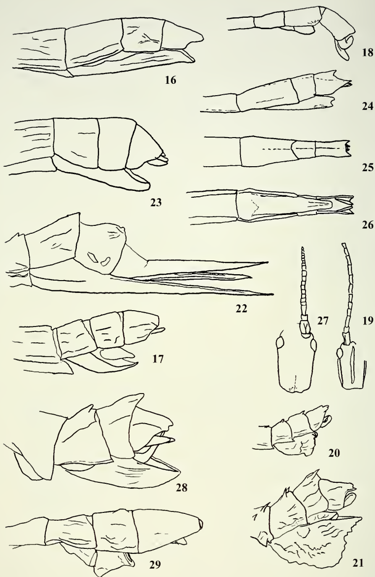
FIGS 16-29. Terminal abdominal segments, lateral aspect. To various scales. Asceles malaccae (Saussure, 1868). 16. HT, ♀. Alloeophasma poeyi (Saussure, 1868). 17. HT, ♀. Gratidia pulchrepecta Carl, 1913. 18. HT, ♂. 19. Head, dorsal aspect. Cnipsus rhachis (Saussure, 1868). 20. ST, ♂. 21. ST, ♀. Labidiophasma rouxi Carl, 1915. 22. ST, ♀. Marmessoidea rubescens (Saussure, 1868). 23. HT, ♀. Paraleptinia schulthessi (Carl, 1913). 24. HT, ♀. 25. Dorsal aspect. 26. Ventral aspect. 27. Head, dorsal aspect. Andropromachus scutatus Carl, 1913. 28. HT, ♀. Pseudostheneboea segregata Carl, 1913). 29. HT, ♂.
