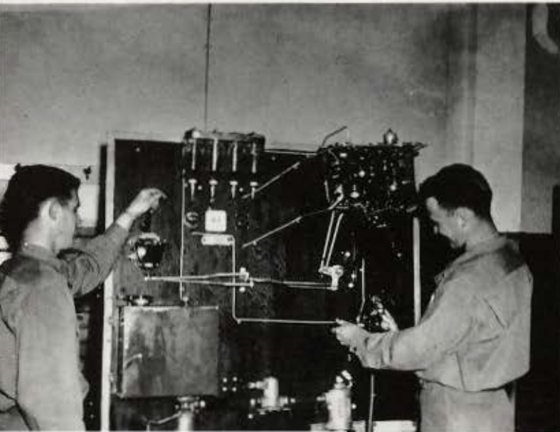
Mockup, Fuel System.
