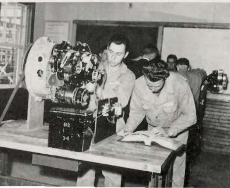
Starter, Engine Accessory Section.
