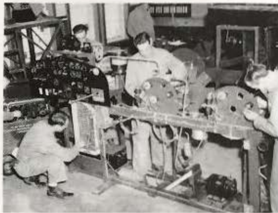
Mockup, Instrument System.
