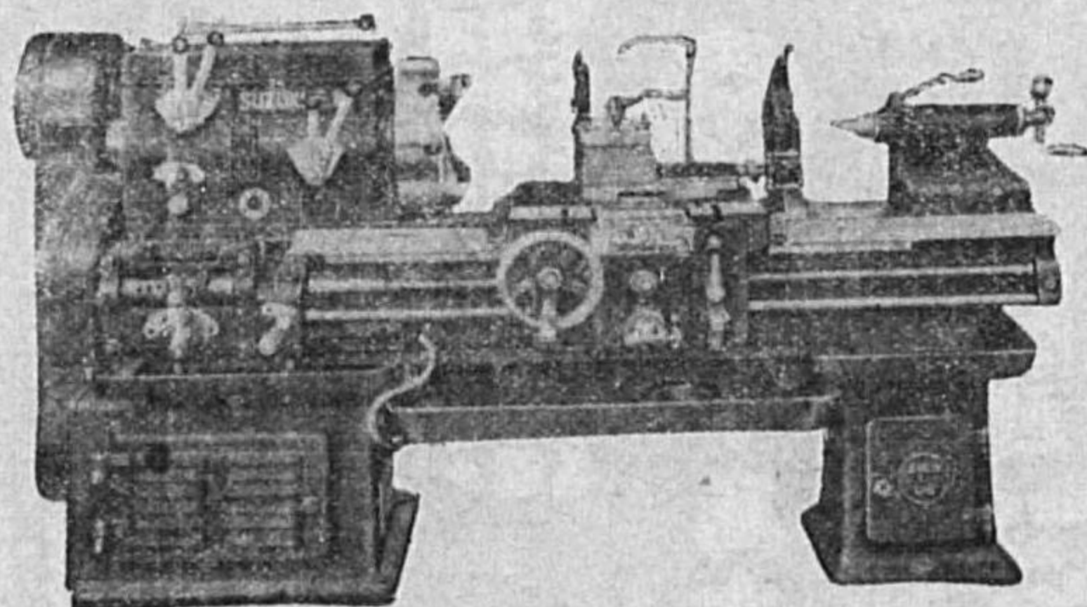
LC TYPE 200 x 1,950 ALL-GEARED PRECISION POWER METRIC LATHE
