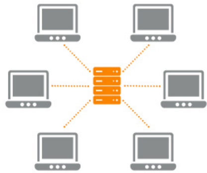
Server-Based
