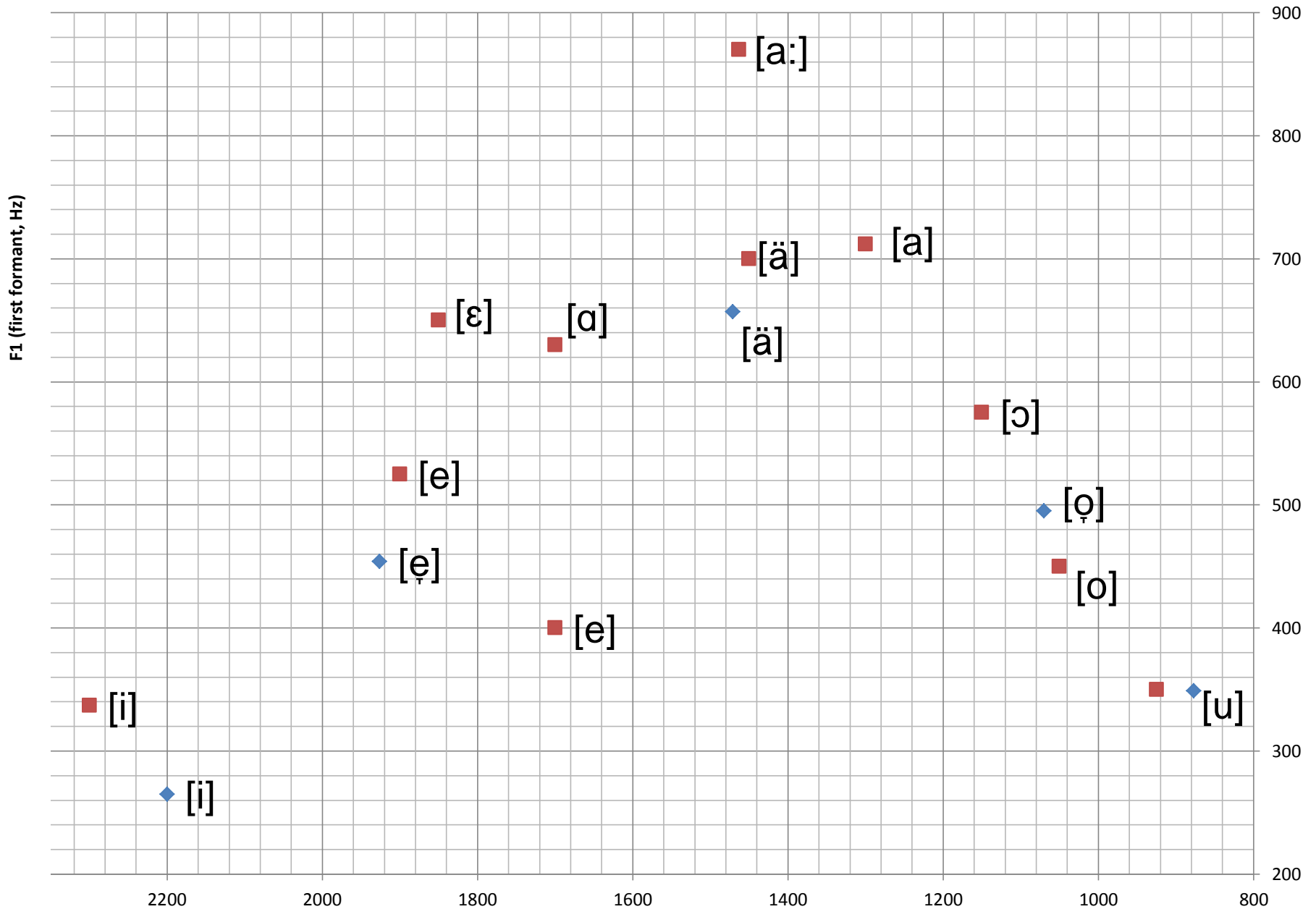
F2 (second formant Hz)
