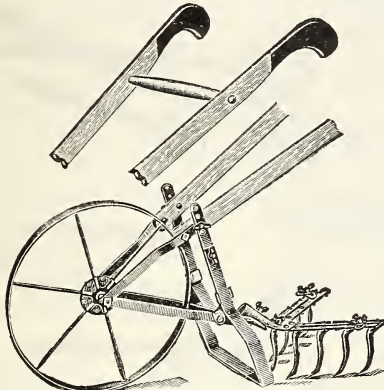
No. 2 Pull Easy Wheel Cultivator.
