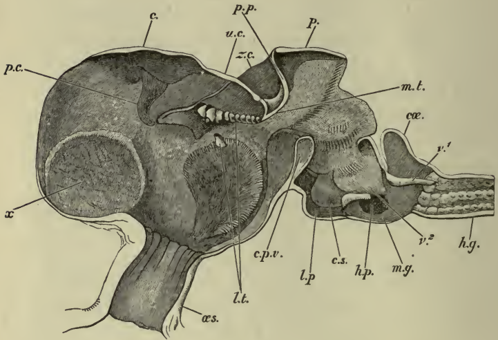
FIG. 10.— Astacus fluviatilis .—Longitudinal section of the stomach ( \times 4 ). c , cardiac ossicle; cœ , cæcum; c.p.v. , cardio-pyloric valve; cs , cushion-shaped surface; hg , hind-gut; hp , aperture of right bile duct; lp , lateral pouch; lt , lateral teeth; mg , mid-gut; mt , median tooth; æs , oesophagus; p , pyloric ossicle; pc , pterocardiac ossicles; pp , prepyloric ossicle; uc , urocardiac process; v 1 , median pyloric valve; v 2 , lateral pyloric valve; x , position of gastrolith; zc , zygocardiac ossicle.
