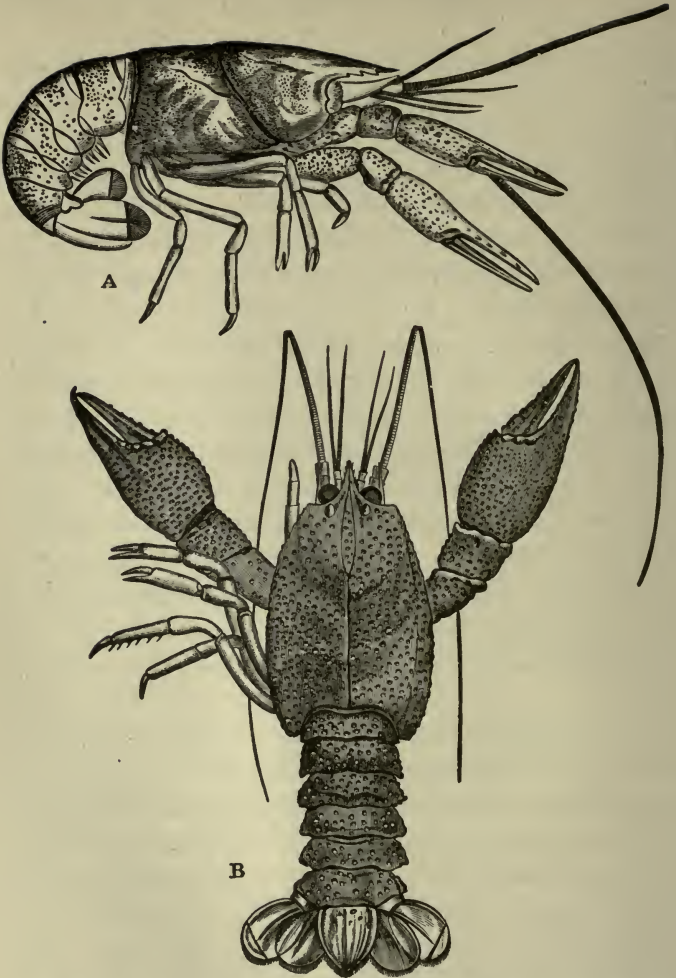
FIG. 80.—A, Pseudastacus pustulosus (nat. size). B, Eryma modesta formis ( \times 2 ). Both figures after Oppel.
