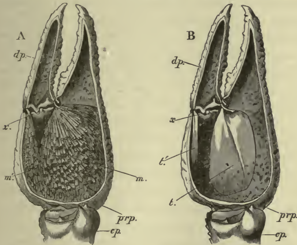
FIG. 20.— Astacus fluviatilis .—The chela of the forceps, with one side cut away to show, in A, the muscles, in B, the tendons ( \times 2 ). cp , carpodite; prp , propodite; dp , dactylopodite; m , adductor muscle; m' , abductor muscle; t , tendon of adductor muscle; t' , tendon of abductor muscle; x , hinge.
