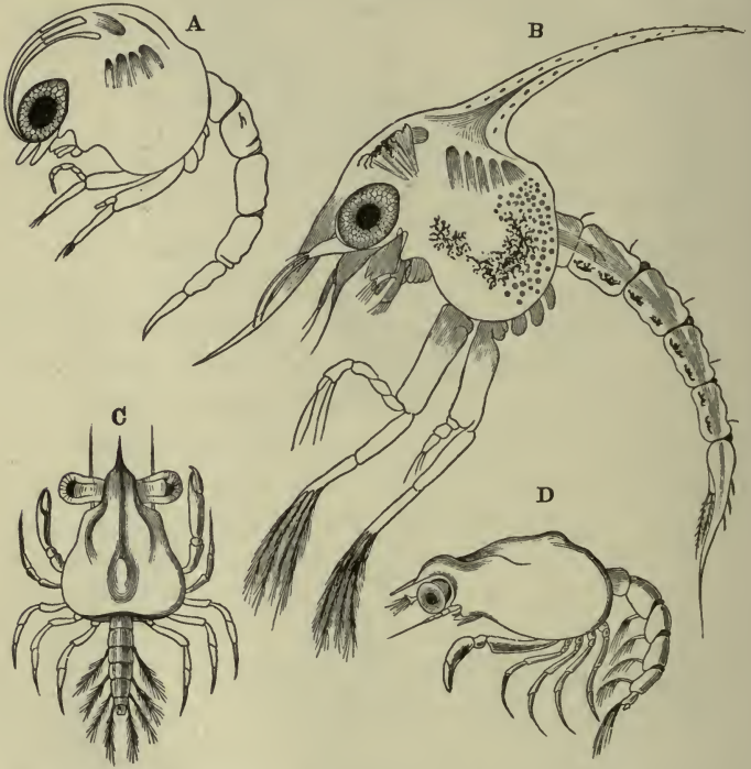
FIG. 74. Cancer pagurus . A, newly hatched Zoæa; B, more advanced Zoæa; C, dorsal, and D, side view of Megalopa (after Spence Bate). The figures A and B are more magnified than C and D.)
