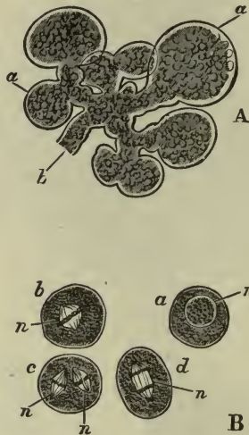
FIG. 33.— Astacus fluvialtilis .—A, a lobule of the testis, showing a , acini, springing from b , the ultimate termination of a duct ( \times 50 ). B, spermatic cells; a , with an ordinary globular nucleus n ; b , with a spindle-shaped nucleus; c , with two similar nuclei; and d , with a nucleus undergoing division ( \times 600 ).
