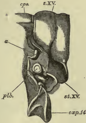
FIG. 38. — Astacus fluviatilis .—The mode of connexion between the last thoracic and the first abdominal somites ( \times 3 ). a , L-shaped bar; cpe , carapace; cxp. 14 , coxopodite of the last ambulatory leg; plb. , place of attachment of the pleurobranchia; st. XV , sternum, and t. XV , tergum of the first abdominal somite.
