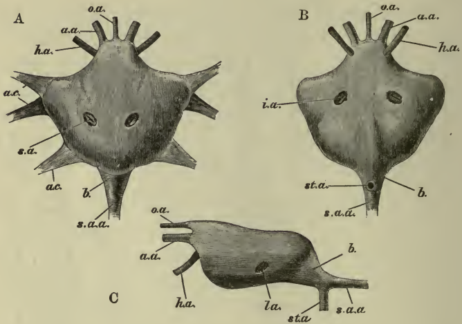
FIG. 16.— Astacus fluviatilis .—The heart ( \times 4 ). A, from above; B, from below; C, from the left side. aa , antennary artery; ac , alae cordis, or fibrous bands connecting the heart with the walls of the pericardial sinus; b , bulbous dilatation at the origin of the sternal artery; ha , hepatic artery; la , lateral valvular apertures; oa , ophthalmic artery; sa , superior valvular apertures; s.a.a , superior abdominal artery; st.a , sternal artery, in B cut off close to its origin.
