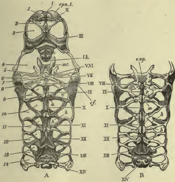
FIG. 39.— Astacus fluviatilis .—The cephalothoracic sterna and the endophragmal system ( \times 2 ). A , from beneath; B , from above. a, a' , arthrophragms or partitions between the articular cavities for the limbs; c.ap. , cephalic apodeme; cf. , cervical fold; epn. 1 , epimeron of the antennulary somite; h , anterior, and h' , posterior horizontal process of endopleurite; lb. , labrum; m , mesophragm; mt. , metastoma; p , paraphragm; 1—XIV , cephalothoracic sterna; 1—14 , articular cavities of the cephalothoracic appendages. (The anterior cephalic sterna are bent downwards in A so as to bring them into the same plane with the remaining cephalothoracic sterna; in B these sterna are not shown.)
