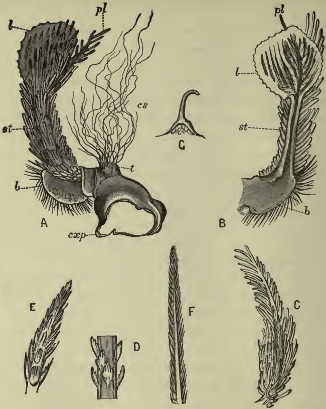
FIG. 17. — Astacus fluviatilis .—A, one of the podobranchiæ from the outer side ; B, the same from the inner side ; C, one of the arthrobranchiæ ; D, a part of one of the coxopoditic setæ ; E, extremity of the same seta ; F, extremity of a seta from the base of the podobranchia ; G, hooked seta of the lamina ; (A—C, \times 3 ; D—G, highly magnified). b , base of podobranchia ; cs , coxopoditic setæ ; cxp , coxopodite ; l , lamina, pl , plume, and st , stem of podobranchia ; t , tubercle on the coxopodite, to which the setæ are attached.
