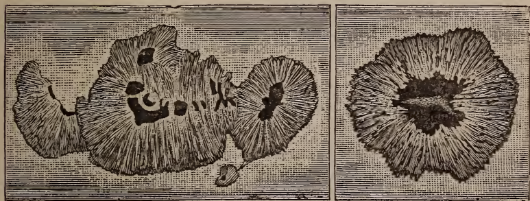
Fig. 20. Solar Spots.
