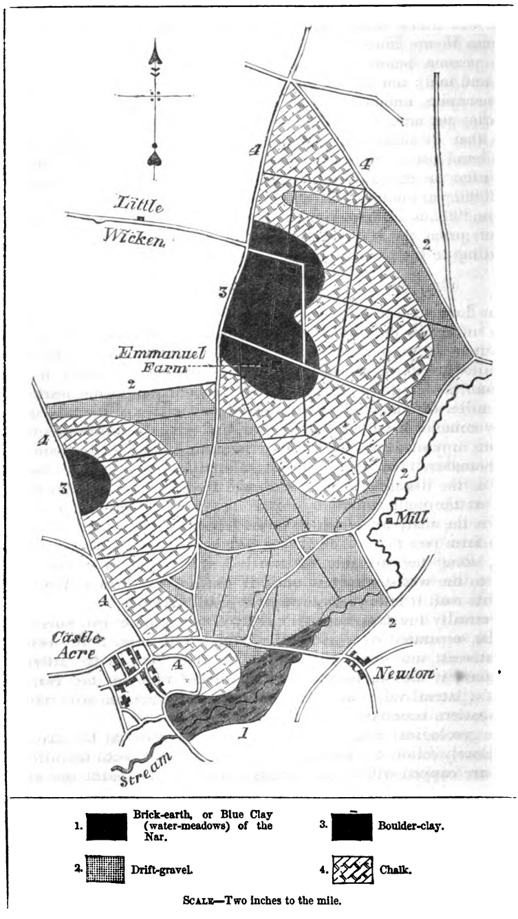
Fig. 1.—Geological Map of the Lodge (or Emmanuel) Farm, Castle Acre.
