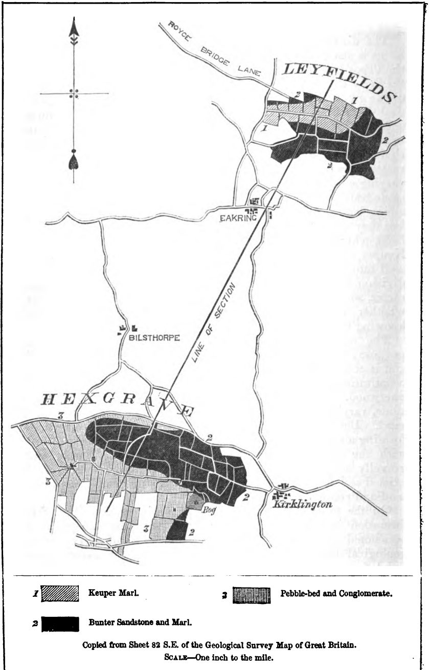
Fig. 1.—Geological Map of Hexgrave and Leyfields.
