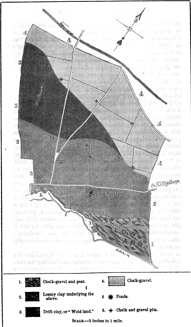
Fig. 1.—Map of Eastburn Farm, near Driffield, showing the Surface Geology After a Survey by J. R. MORTIMER, Esq.
