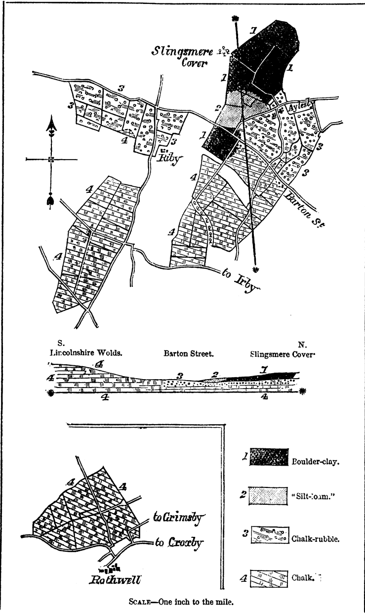
Fig. 1.—Geological Map of the Farms occupied by Mr. TORR at Aylesby, Riby, and Rothwell.
