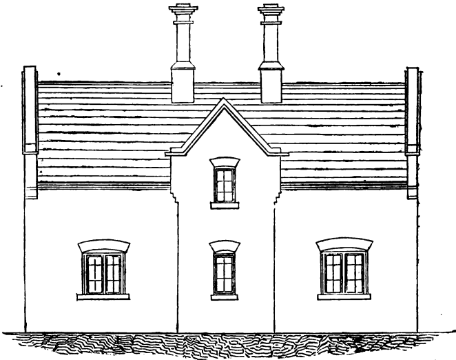
Fig. 3.— Front Elevation of a pair of Labourers' Cottages at Aylesby.
