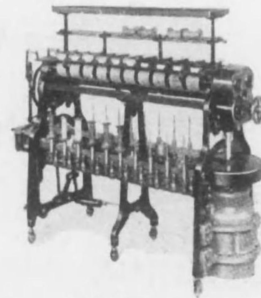
Single deck Granedine Twister
