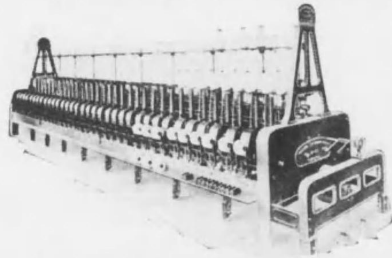
PATENT VERTICAL BURNER GASSING FRAME DOWNWARD EXHAUST TYPE.
