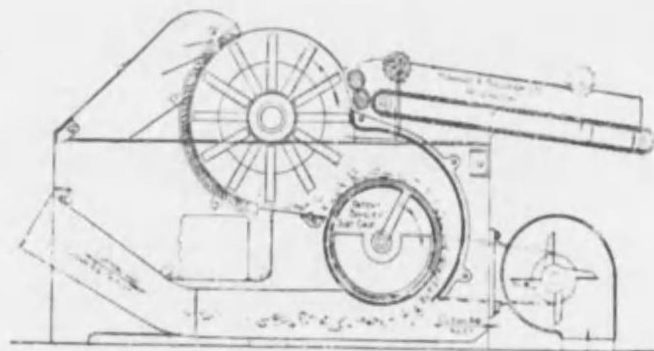
Patent "Shirley" High Speed Cage as applied to Opener with 24" Porcupine Cylinder
