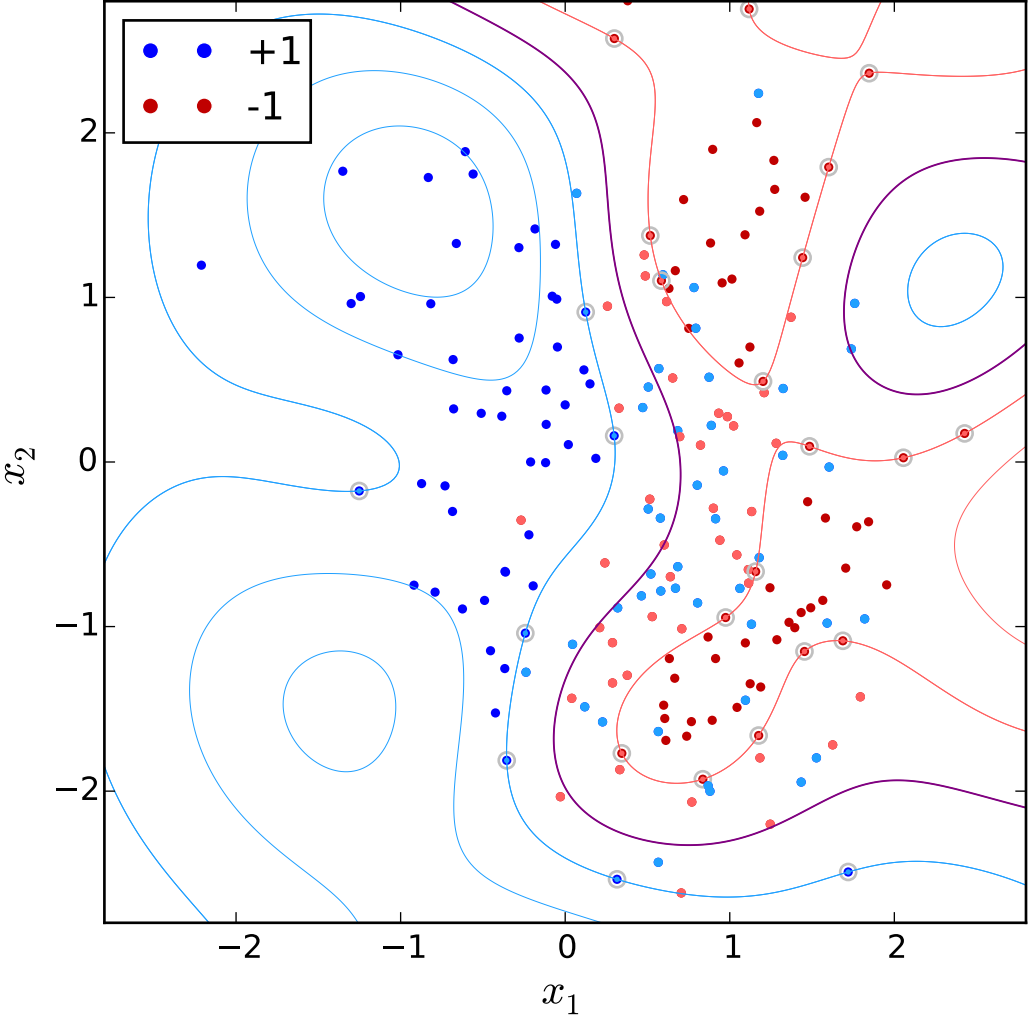
gaussian kernel
