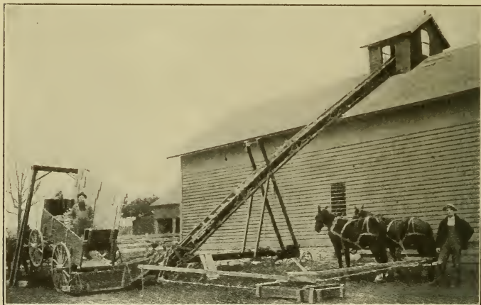
FIG. 84.—A good type of farm corn crib, and farm elevator used in unloading.
