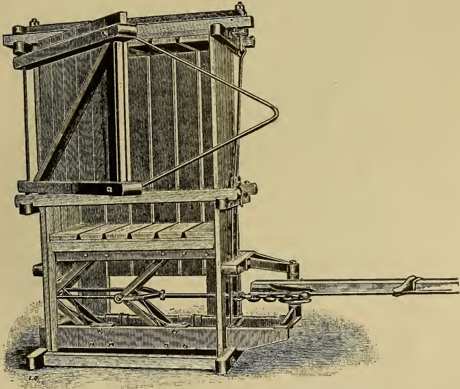
FIG. 119. — Power baling press for broom-corn.
