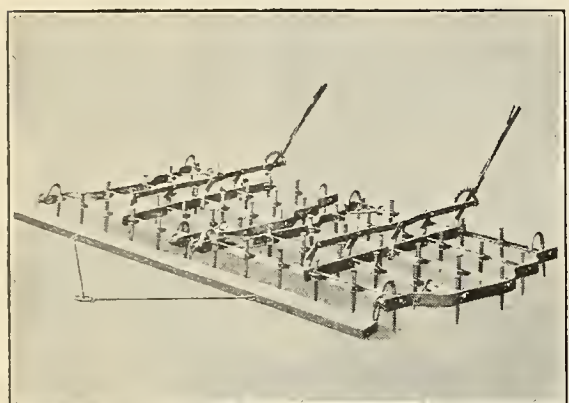
Ohio Spike Tooth Harrow
