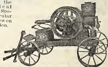
Deyo Hopper Cooled Engine.
