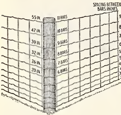
Top and Bottom No. 9 "JUMBO" FENCE
