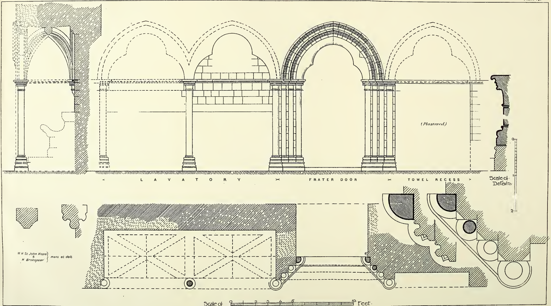
ROCHESTER PRIORY—FRATER DOOR & REMAINS OF LAVATORY, ETC.
