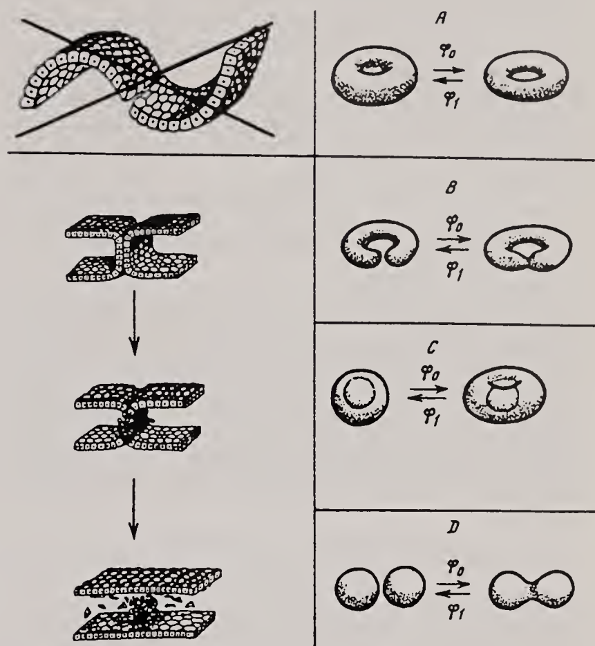
Fig. 2 - Modifications (surgery) of topology during embryonic pattern formation. Left column: local aspect of surgeries; Right column: global aspects of surgeries. \varphi_0, \varphi_1 - surgeries. A_{\varphi_0} - oral plate rupture; A_{\varphi_1} - obliteration of branchial clefts; B_{\varphi_0} - obliteration of choroid fissure; B_{\varphi_1} - separation of somites from splanchnotome; C_{\varphi_0} - mouth breaking into blind archenteron; C_{\varphi_1} - neurulation; D_{\varphi_0} - fusion of two heart anlagen, formation of a single body cavity when the sheets of lateral plate fuse; D_{\varphi_1} - enterocoel mode of the formation of the mesoderm.
