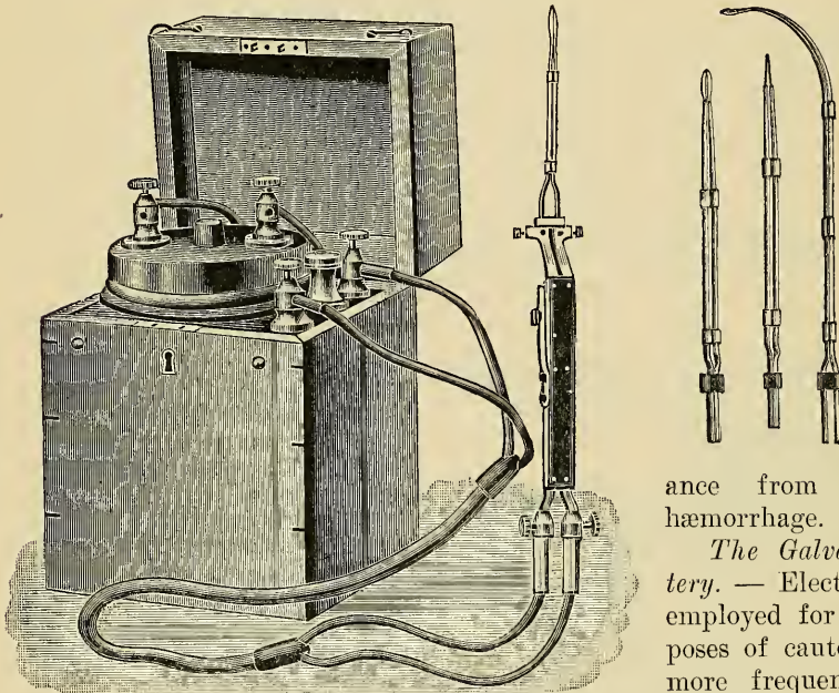
FIG. 109.—Galvano-cautery battery, with knife electrodes.
