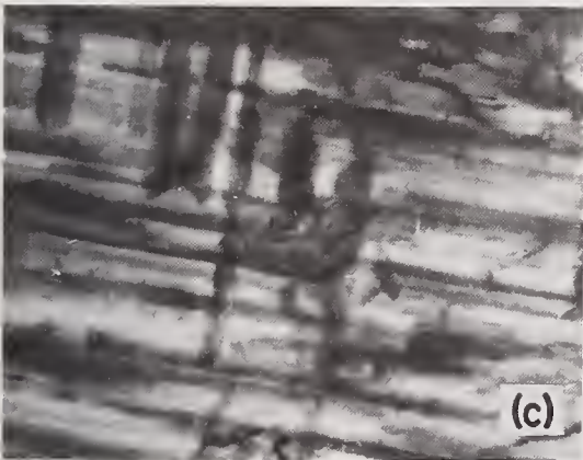
Fig. A.6. Various kinds of structural defects observed in (100) silicon diffused with high amounts of phosphorus. (a) Dislocation loops are formed in initial diffusion stage. (b) Dislocation nets are formed after interaction within loop dislocations in final diffusion state. (c) Thin precipitate platelets of phosphorus-silicon complexes are often observed in diffused layers.
