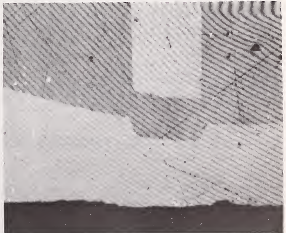
Fig. 10. Emitter-dip effect in n-p-n structure, photograph courtesy of R. J. Jaccodine.
