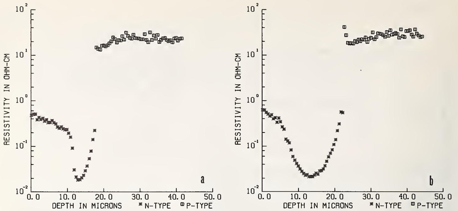
Fig. 9. Resistivity profiles of a buried layer structure from spreading resistance measurements. The profile is through the epitaxial n-layer and the buried n^+ layer to the p substrate: a) immediately after epitaxial deposition; b) after p-wall drive diffusion.
