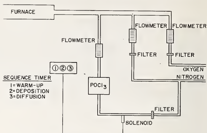
Fig. 15 - Schematic diagram of present POCl_3 system.
