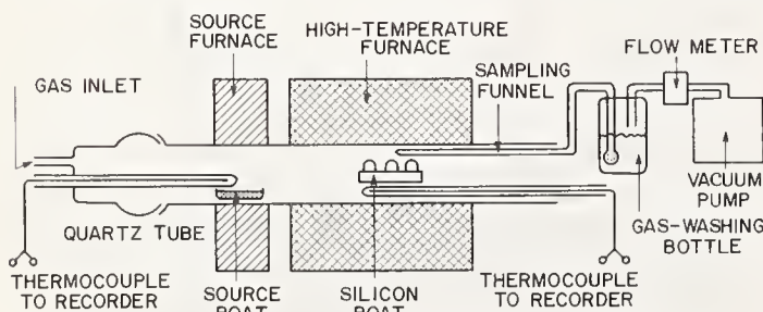
Fig. 1 - Schematic diagram of experimental apparatus.
