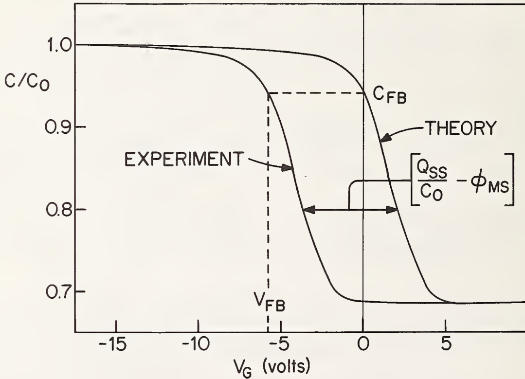
Fig. 1. Typical examples of MOS structures (upper left), C-V curves for p - and n -type silicon (upper right), and measurement of Q_{SS} using MOS C-V plot (bottom). Note that for this and subsequent figures, C_B \sim 1 \times 10^{16} \text{ cm}^{-3} , silicon orientation is (111) and X_0 = 0.2 \mu , unless otherwise specified.
