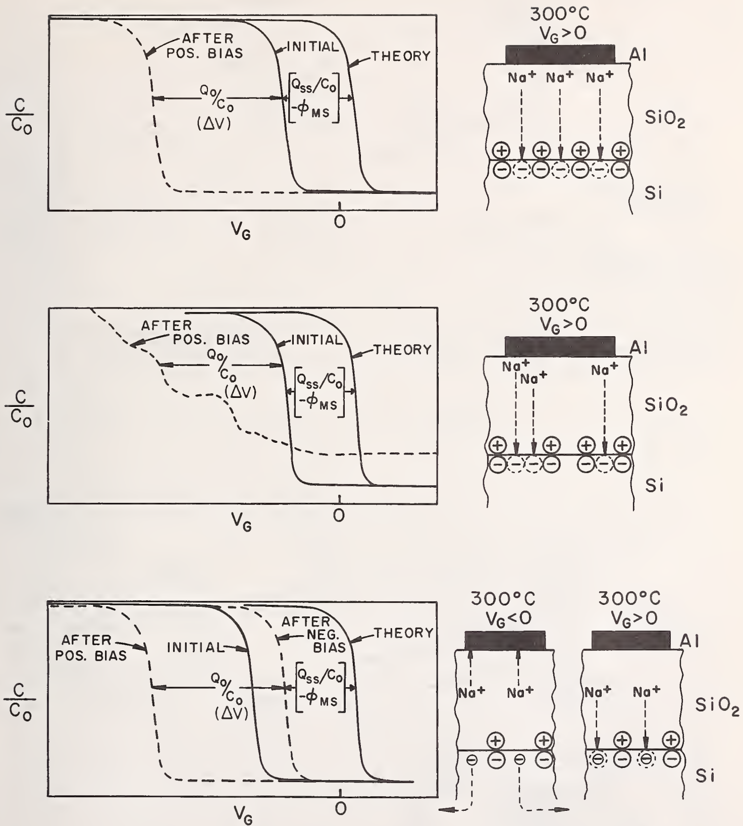
Fig. 2. Examples of three types of ion ( Na^+ ) drift as indicated by MOS C-V plots.
