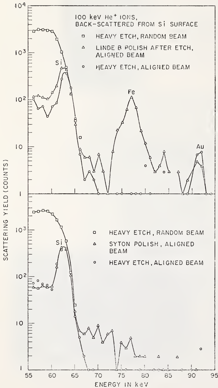
Fig. 9. Scattering Yield vs. Energy of He + Ions Back Scattered from Etched and Syton Polished Silicon Surfaces.
