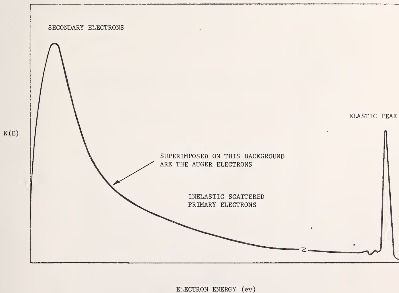
Figure 2 Electron Energy Distribution Curve
