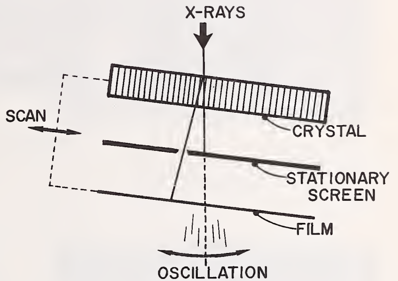
Fig. B.2. Transmission SOT method of Schwuttke. Crystal and film scan and oscillate to record large area topographs in preserve of wafer strain.
