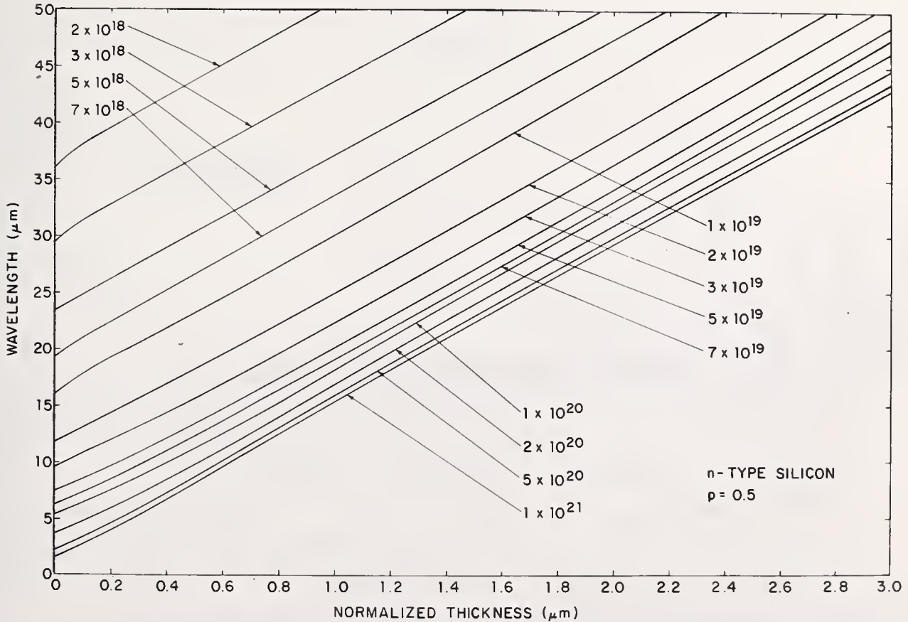
Fig. 5. Wavelength position of order 0.5 minimum as a function of normalized thickness for n/n+ silicon and various substrate carrier concentrations.
