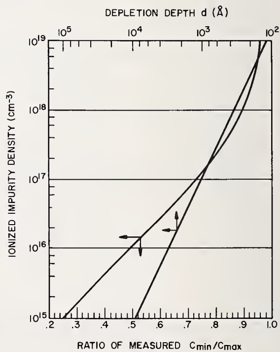
Fig. 5. Calculated ratio of measured C_{min} to C_{max} and also depletion depth of an MIS capacitor on Si with 1000 Å SiO 2 as a function of ionized impurity density.
