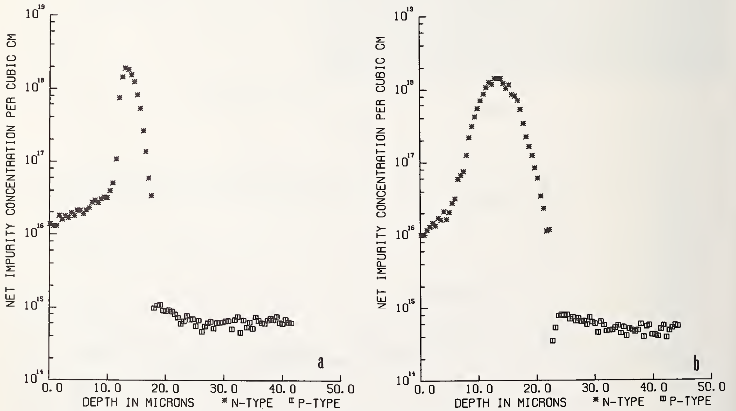
Fig. 10. Carrier concentration profiles corresponding to the resistivity profiles shown in Fig. 9: a) immediately after epitaxial deposition; b) after p-wall drive diffusion.
