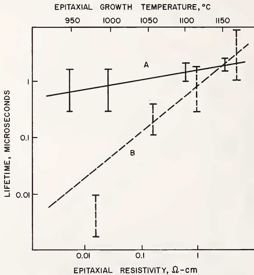
Fig. 7. Comparison of Minority Carrier Lifetime in Epitaxial Silicon Line A - As a Function of Growth Temperature Line B - As a Function of Epitaxial Resistivity
