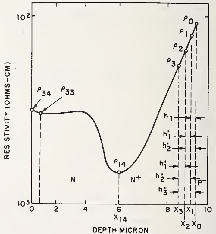
Fig. 10. Initial resistivity values vs. depths for N/N+/P - structure.
