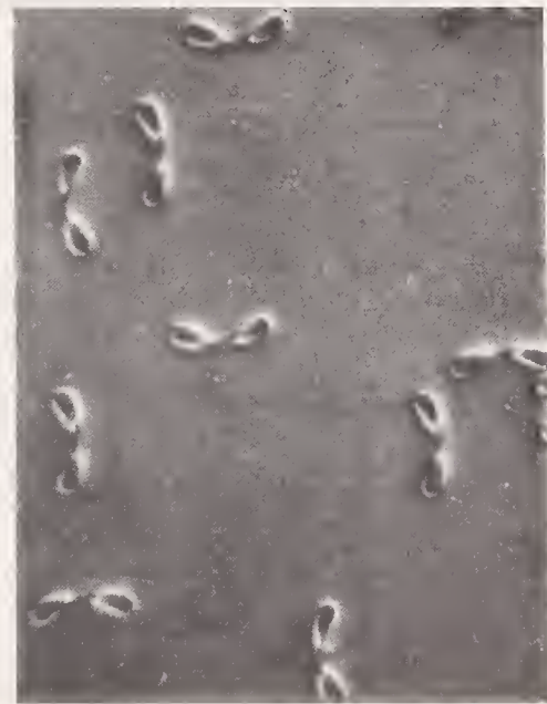
Fig. 6(a) - Differential interference micrograph of silicon surface after stripping 1.0 μm of 1100°C steam grown oxide and Sirtl etching. 360 x
