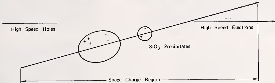
(a) Symmetrical System (Large Spherical \text{SiO}_2 Particle)
