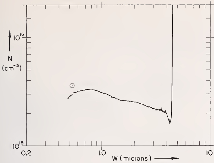
Fig. 5. Doping profile of silane grown epitaxy (1000 °C, 0.25 \mu /min.). Note lighter doped region at NN + interface.
