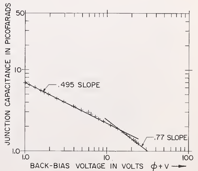
Fig. 8. Log C vs. log V plot of discrete C-V data for material whose doping profile is shown in Fig. 7.
