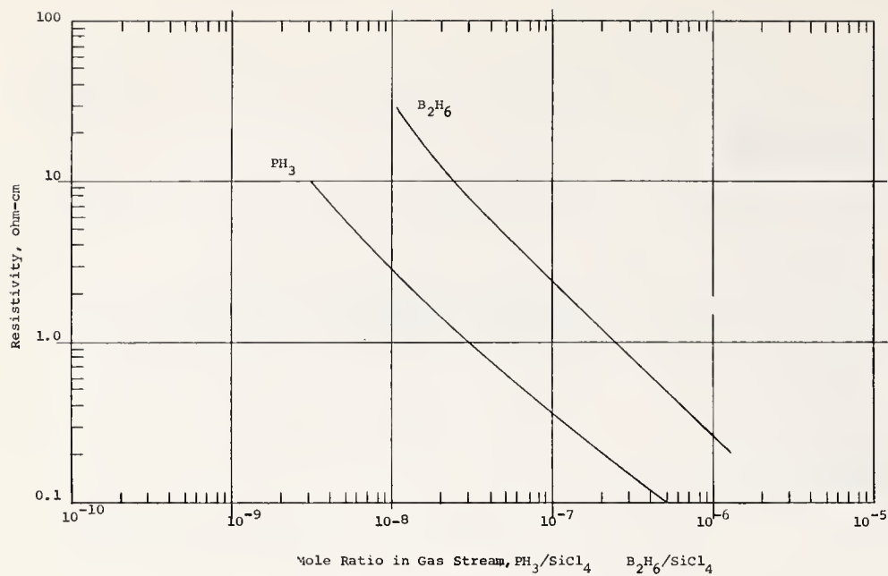
Fig. 3. Film Resistivity vs Dopant gas to \text{SiCl}_4 ratio for Huggle Industries Horizontal Displacement Flow Reactor
