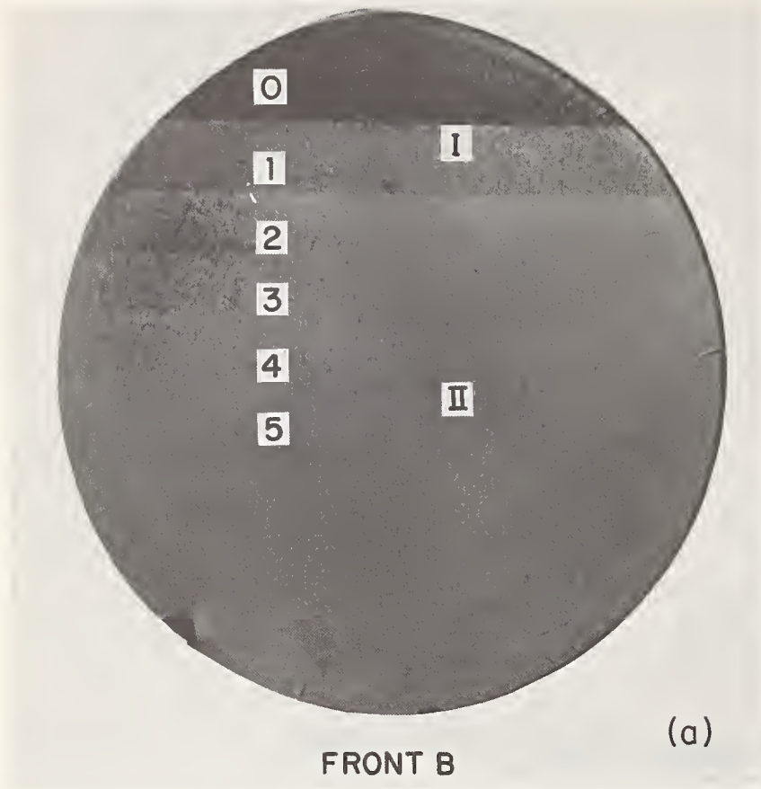
Fig. C.4a. SOT topograph of saw damage in the B surface of wafer cut from front of the crystal. Note contrast reduction after initial step. Damage zones (I) and (II) represent two different modes of saw damage. (See text.)
