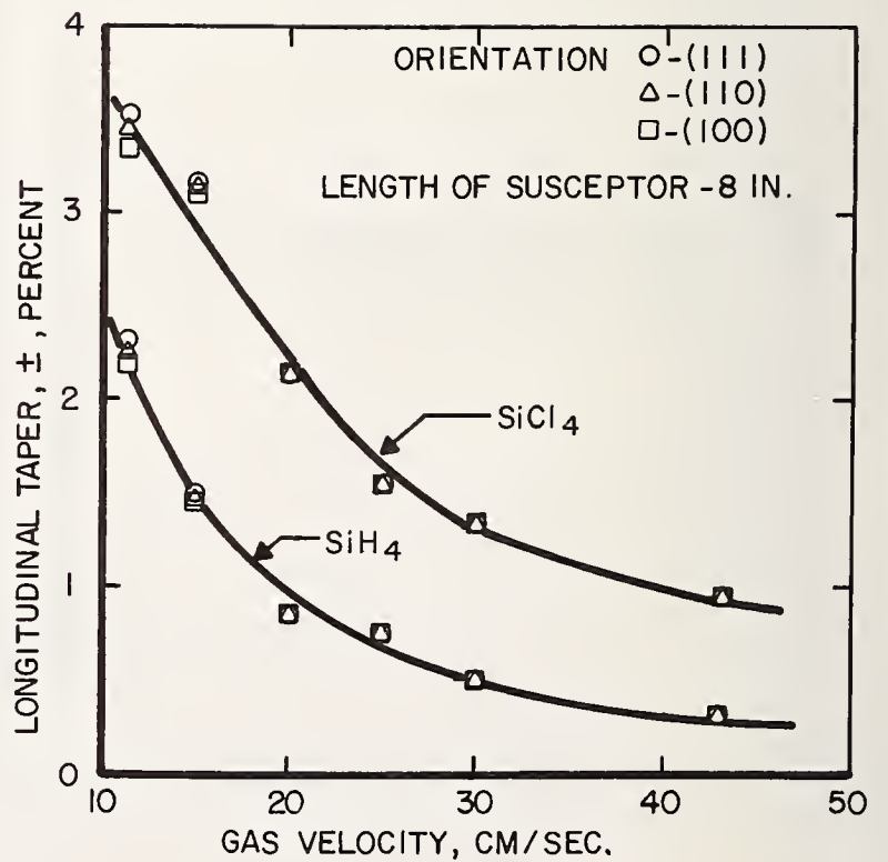
Fig. 8. Longitudinal taper vs. gas velocity in the rectangular tube configuration.
