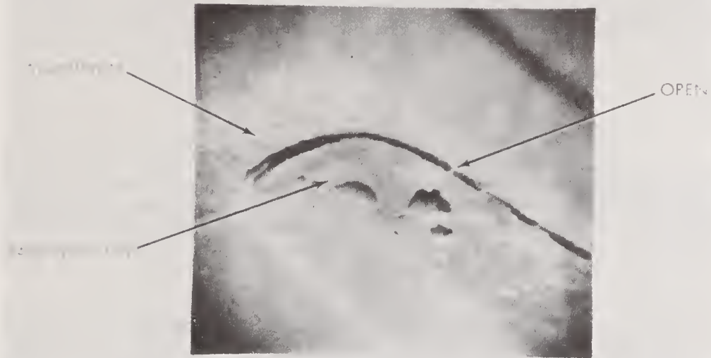
Alumina with Definite Electrical Discontinuities, Mag. 2200 X
