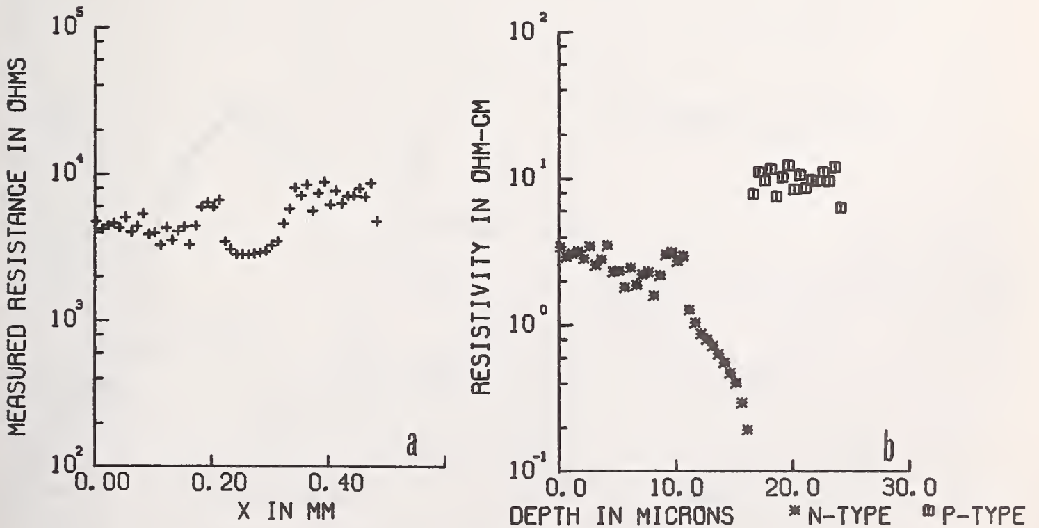
Fig. 12. Profile through an abnormal buried layer region on the same wafer as that used for the data in Fig. 11: a) measured spreading resistance profile; b) resistivity profile from the data in Fig. 12a.
