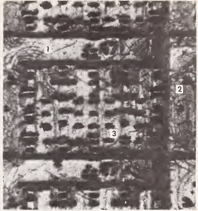
Fig. B.7. Enlargement of A in Fig. B.6. Note dislocation loops (1) which are located near edge of the isolation region and (2) which occur between adjacent chips.
