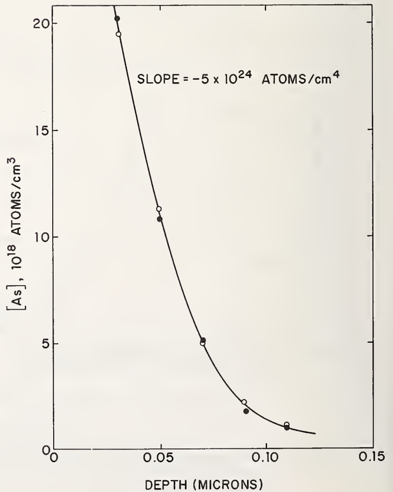
Fig. 7. Radiochemical profiles obtained from wafer diffused with 74 AS-labeled arsenic, following 24 hr. activation with 1 \times 10^{13} thermal neutrons/cm 2 -sec. and post-activation anneal for 30 min. at 625 °C. Profile determined from 74 AS radio-tracer (closed circles) and from 76 AS activation (open circles).
