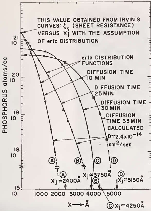
Fig. 1. Phosphorus distribution obtained through open-tube diffusion processes. Observe the reduction of C_s after exceeding x_j \approx 3750 \text{ \AA} .
