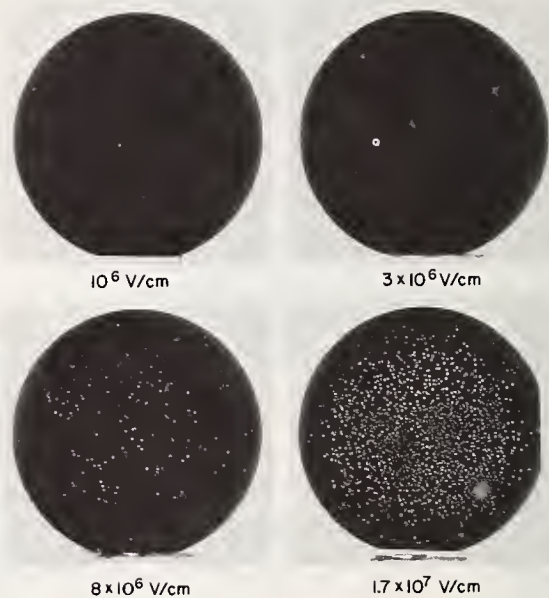
Fig. 9 - Silicon wafer with 1000\text{ \AA} of thermally grown \text{SiO}_2 decorated with copper at successively higher field strengths.
