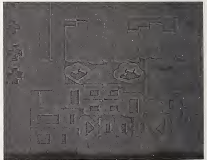
Fig. 8. Pattern washout in an epitaxial wafer. [111] direction oriented 1° from surface normal.
