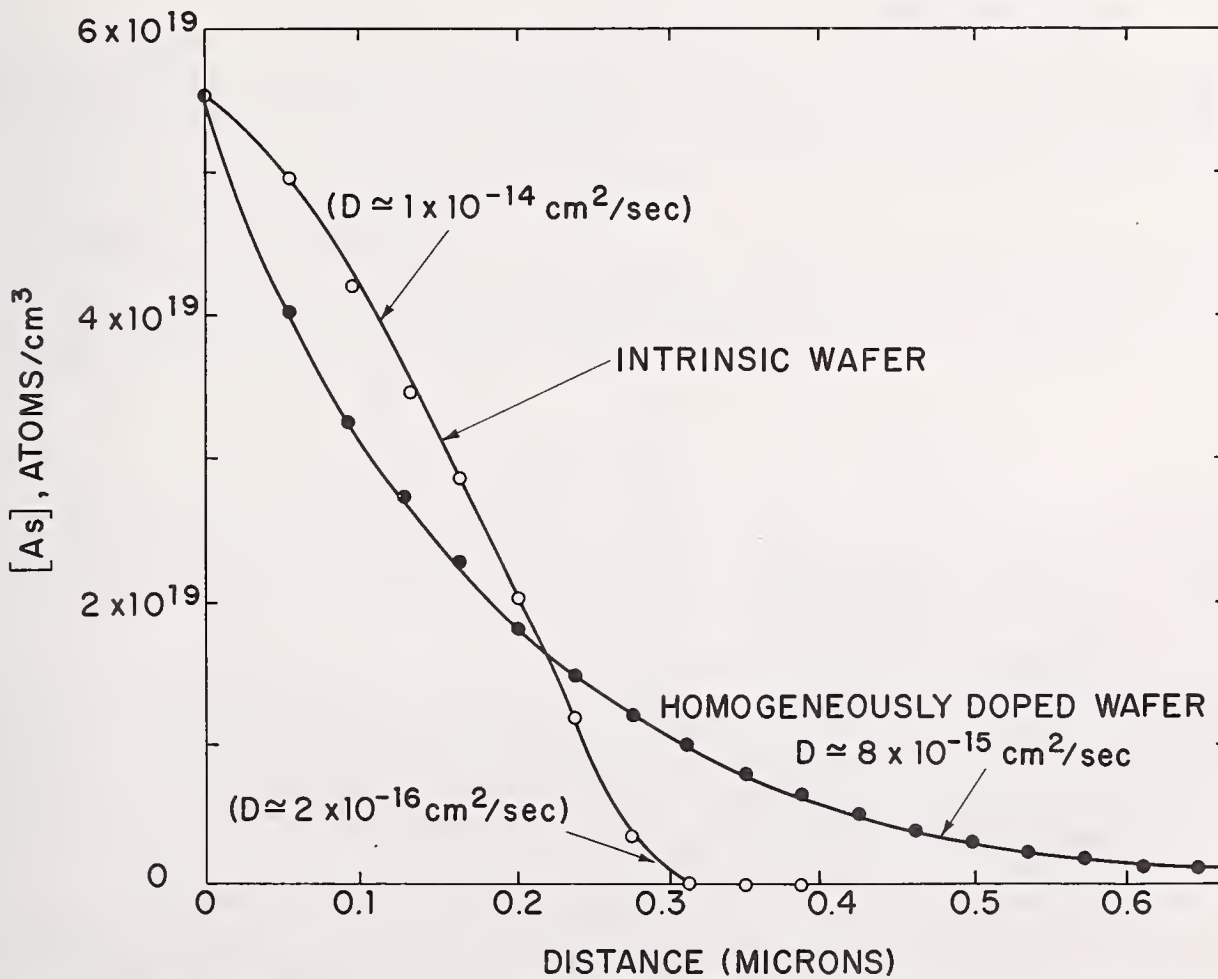
Fig. 5. Radiotracer diffusion of ^{76}\text{As} -labeled arsenic into initially intrinsic silicon (open circles) and into silicon homogeneously doped with 5.5 \times 10^{19} \text{ As-atoms}/\text{cm}^3 (closed circles), both 19 1/2 hrs. @ 956^\circ\text{C} .
