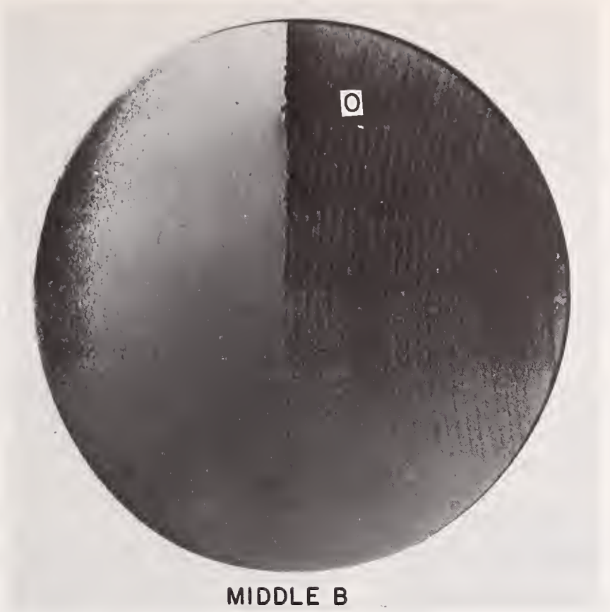
Fig. C.7a. SOT topograph of saw damage in B. surface (middle).
