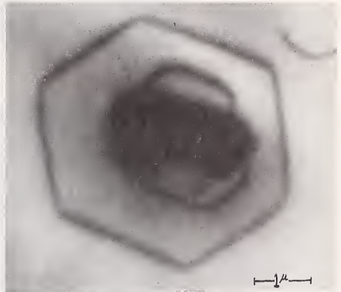
Fig. A.8. Formation of dislocation loops in heat-treated silicon after development of a large SiO 2 particle.
