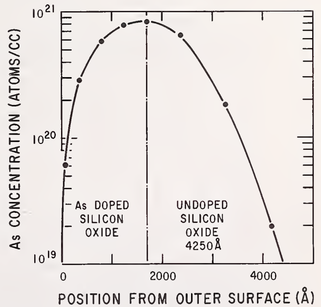
Fig. VIII. Arsenic doped deposited silicon oxide used as a diffusion source. C_s on silicon was 2 \times 10^{17} atoms/cc after diffusion.
