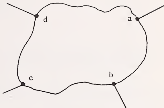
Fig. 7. Van der Pauw geometry. [Ref. 11]
