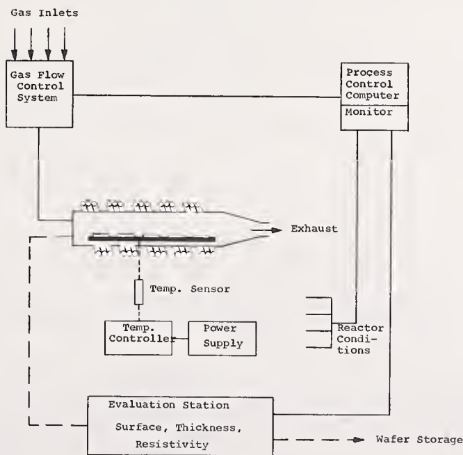
Fig. 6. Automatic Program Controlled Batch Epitaxial Reactor System.
