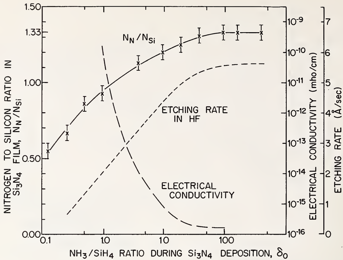
Fig. 12. Relationship among silicon nitride film composition, etch rate, and conductivity as influenced by \text{NH}_3/\text{SiH}_4 ratio during nitride deposition [50].
