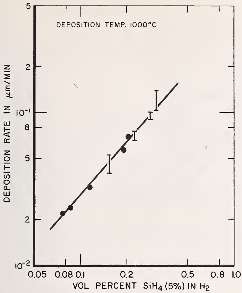
Fig. 1. Effect of SiH 4 -H 2 ratio on the silicon deposition rate using 5 percent SiH 4 mixture in hydrogen (7).
