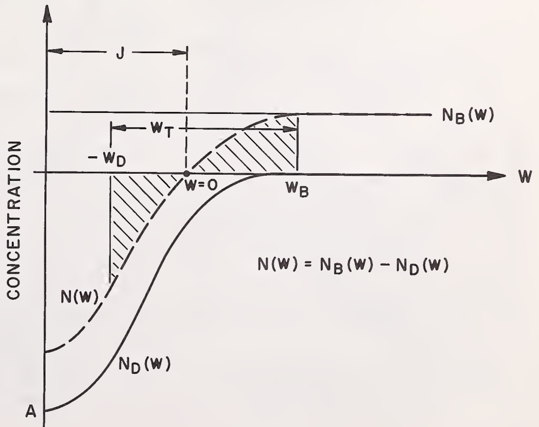
Fig. 4. Model for the calculation of depletion layer widening and compensation near the junction due to the impurity diffusion tail itself.
