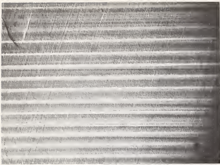
Fig. 5. Top view of the surface of the epitaxial layer shown in Fig. 4. The surface was etched in B-etch to reveal the arrays.
