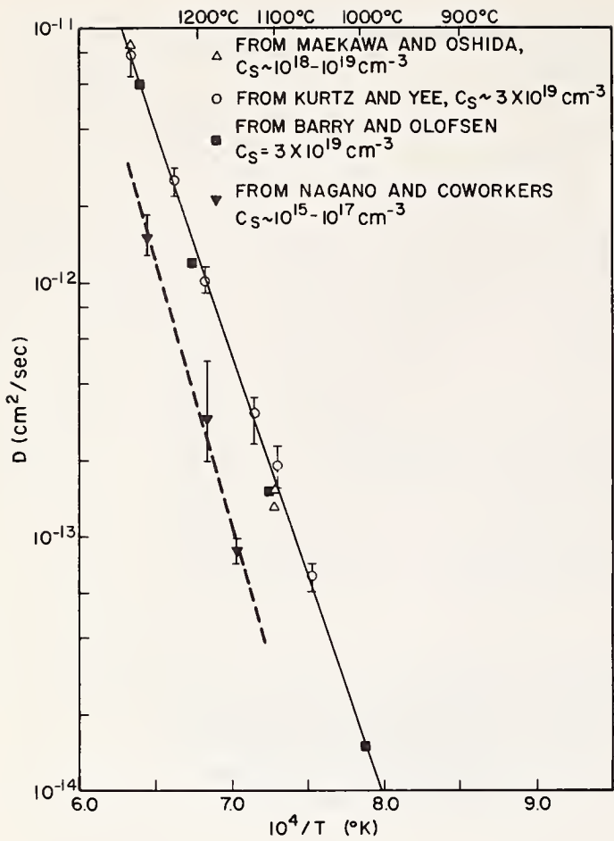
Fig. 7. Diffusion coefficients of boron at low surface concentrations; measurements by Maekawa and Oshida [32], Kurtz and Yee [31], Barry and Olofsen [18], and Nagano and coworkers [19].
