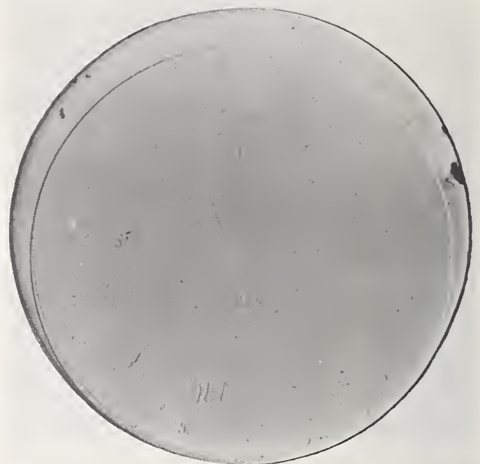
Fig. E.8. Topograph after Al deposition. Note several contrast lobes near edge of film.
