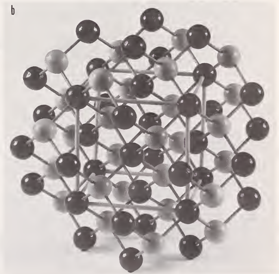
Fig. 6. Views of a diamond-type lattice from (a) a \langle 110 \rangle direction, and (b) 10^\circ off a \langle 110 \rangle direction.
