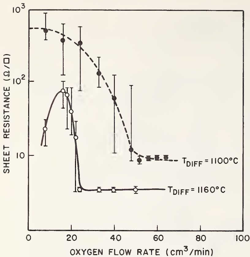
Fig. 3. Sheet resistance versus oxygen flow rate (in a 60 mm I.D. tube) in a diffusion using a \text{BCl}_3 source, from Nakamura [8].
