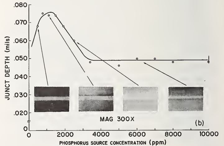
Fig. F.2. Dependence of junction depths in open-tube P-diffusion systems. [83] a. Junction depth vs phosphorus concentration after the deposition cycle only. b. Junction depth vs phosphorus concentration after both the deposition and drive-in-cycle. Photo inserts illustrate the junction depth from beveling and staining at representative points.
