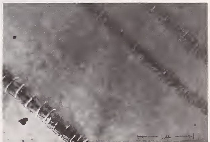
Fig. A.9. Scratches on silicon surfaces have developed into rows of dislocation loops after heat-treatment at 1000 °C.
