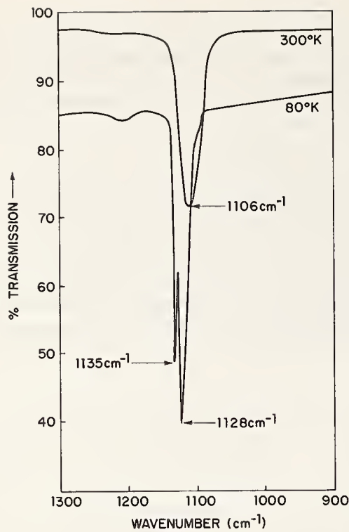
Fig. 1. The 1106 \text{ cm}^{-1} band due to dissolved oxygen at room temperature and at approximately 80 \text{ }^\circ\text{K} . Upon cooling, a band at 1135 \text{ cm}^{-1} becomes visible while the 1106 \text{ cm}^{-1} band shifts to 1128 \text{ cm}^{-1} .
