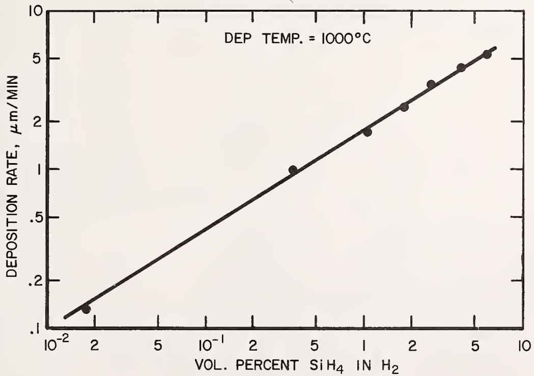
Fig. 2. Effect of SiH 4 -H 2 ratio on the silicon deposition rate using 100 percent SiH 4 .
