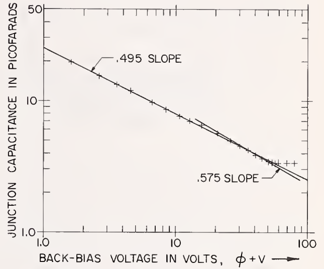
Fig. 6. Log C vs. log V plot of discrete C-V data for material whose doping profile is shown in Fig. 5.
