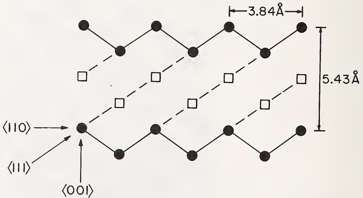
Fig. 8. Cross section of the silicon lattice in the (\bar{1}\bar{1}0) plane, showing substitutional sites (solid circles) and tetrahedral interstitial sites (open squares).
