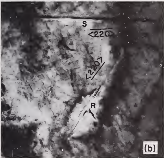
Fig. 5. Precipitates of phosphorus in silicon corresponding to shallow diffusion. Generation of a dislocation patch at the intersection of a precipitate platelet M in (111) silicon corresponding to C-type impurity distribution given in Fig. 1. Structure giving fringe contrast similar to that of a stacking fault. Contrast experiments indicated that these are most probably very thin P-Si precipitates corresponding to the same diffusion as in Fig. 5(a). Singular dislocation node O and clearly identifiable stacking faults P and Q are observed. Clearly identifiable stacking faults, however, were only occasionally observed.
