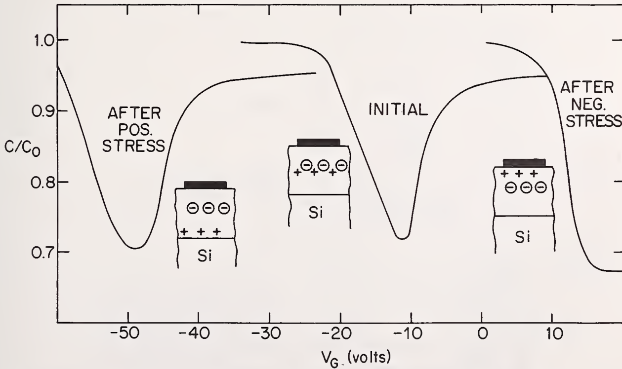
Fig. 7. Example of negative charges remaining in thermal oxide after high temperature contamination. C-V plots show that negative ions do not drift at 300°C resulting in a positive "turn-on" voltage after negative stress at 300°C.
