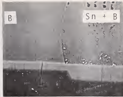
Fig. F.9a. Cooperative diffusion effects. Push-out by diffusing, first Sn; then B.
