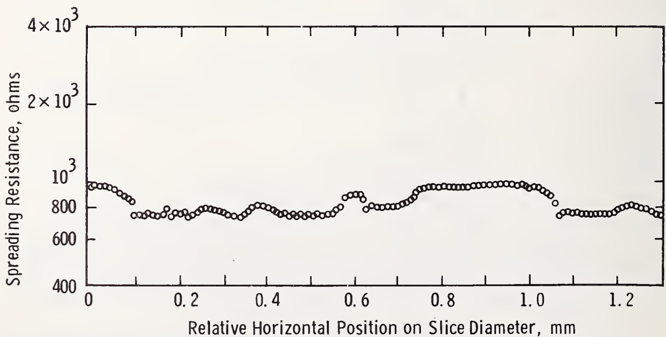
Fig. 6. Spreading resistance profile across part of the an as-grown surface of a wafer containing buried layers. Horizontal step increment ( \Delta X = 10 \mu\text{m} ).
