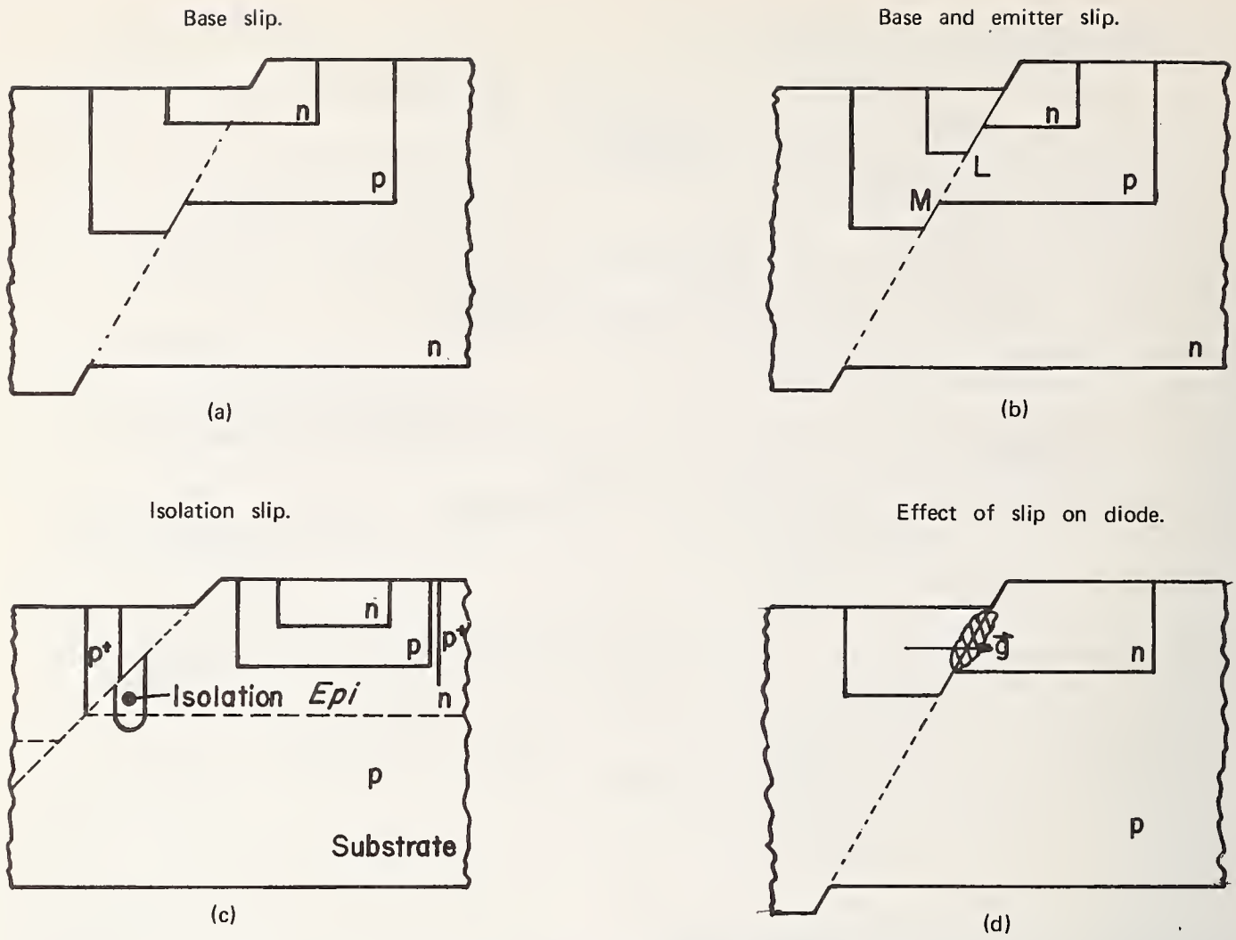
Fig. A.4. Effect of slip on vertical structures of transistors.
