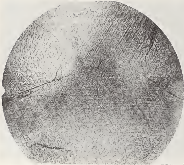
Fig. 4. Topograph of large-diameter \langle 111 \rangle crystal exhibiting high dislocation densities, thermal slip, and lineage.
