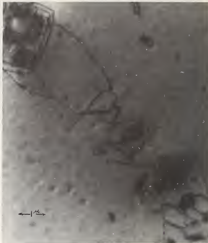
Fig. G.2. Observe dislocation generation around \text{Si}_x\text{O}_y complexes. Dislocations were found purely edge-type. TEM observation, courtesy of Patrick and Dash.
