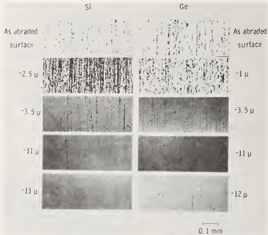
Si and Ge wafer, abraded on 600 Al 2 O 3 , water as lubricant; areas of surfaces after "planar polishing" with 1/4 \mu diamond, 1 sec etched in CP4; depths below max elevation on as abraded surface as indicated.
