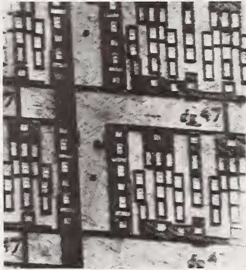
Fig. B.10. Surface x-ray topograph of region in Fig. B.9. Short line segments represent steeply inclined dislocation segments (slip array), which intercept the surface. Note disparity in volume and surface defect density transmission (volume) topograph can exaggerate surface defect density.
