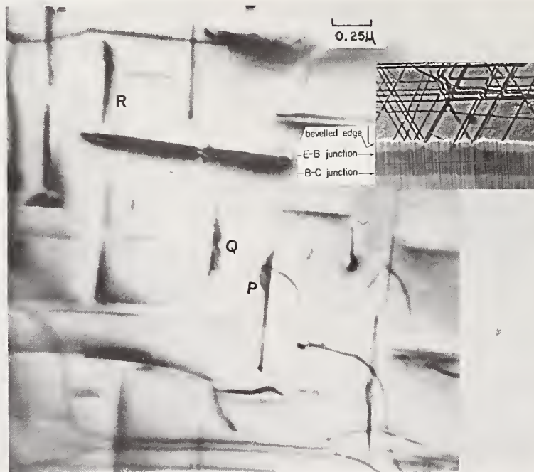
Fig. F.7. Observe diffusion-induced dislocations decorated with phosphorus at P, Q, and R. Right-corner insert in figure shows emitter-base junction (E-B) is seen retarded at every point under the dislocations. Insert, courtesy of Yoshida and Kanamori.
