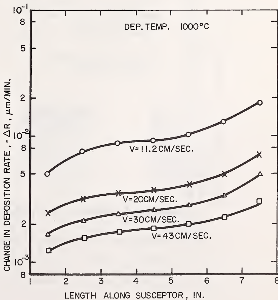
Fig. 10. Longitudinal uniformity as a function of gas velocity for depositions using \text{SiH}_4 in rectangular tube configuration.
