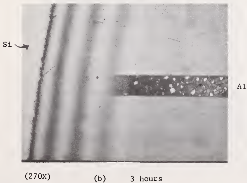
Fig. 8. Beveled Al on SiO 2 on Si Samples Aged at 523 °C.
