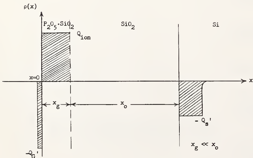
Fig. 6. A Model of the Al-SiO 2 -Si System.
