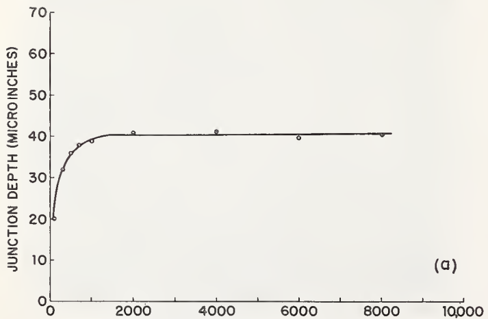
Fig. F.2. Dependence of junction depths in open-tube P-diffusion systems. [83] a. Junction depth vs phosphorus concentration after the deposition cycle only. b. Junction depth vs phosphorus concentration after both the deposition and drive-in-cycle. Photo inserts illustrate the junction depth from beveling and staining at representative points.
