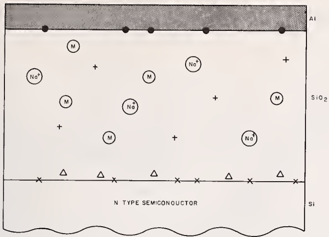
Fig. 1. Classification of States and Charges for the Al-SiO 2 -Si System.
