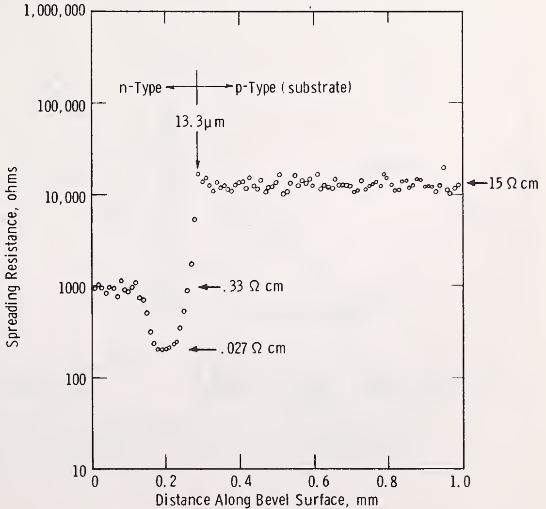
Fig. 8. Spreading resistance profile through both the epitaxial n on p layer and the buried (diffused) n^+ layer: single spreading resistance probe, using a large-area current-return contact and a horizontal step of 10 \mu\text{m} between successive measurement points.
