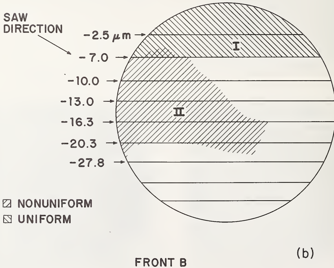
Fig. C.4b. Damage map, front B. Depth of damage indicated after each step is average of ten measurements at different locations along step.
