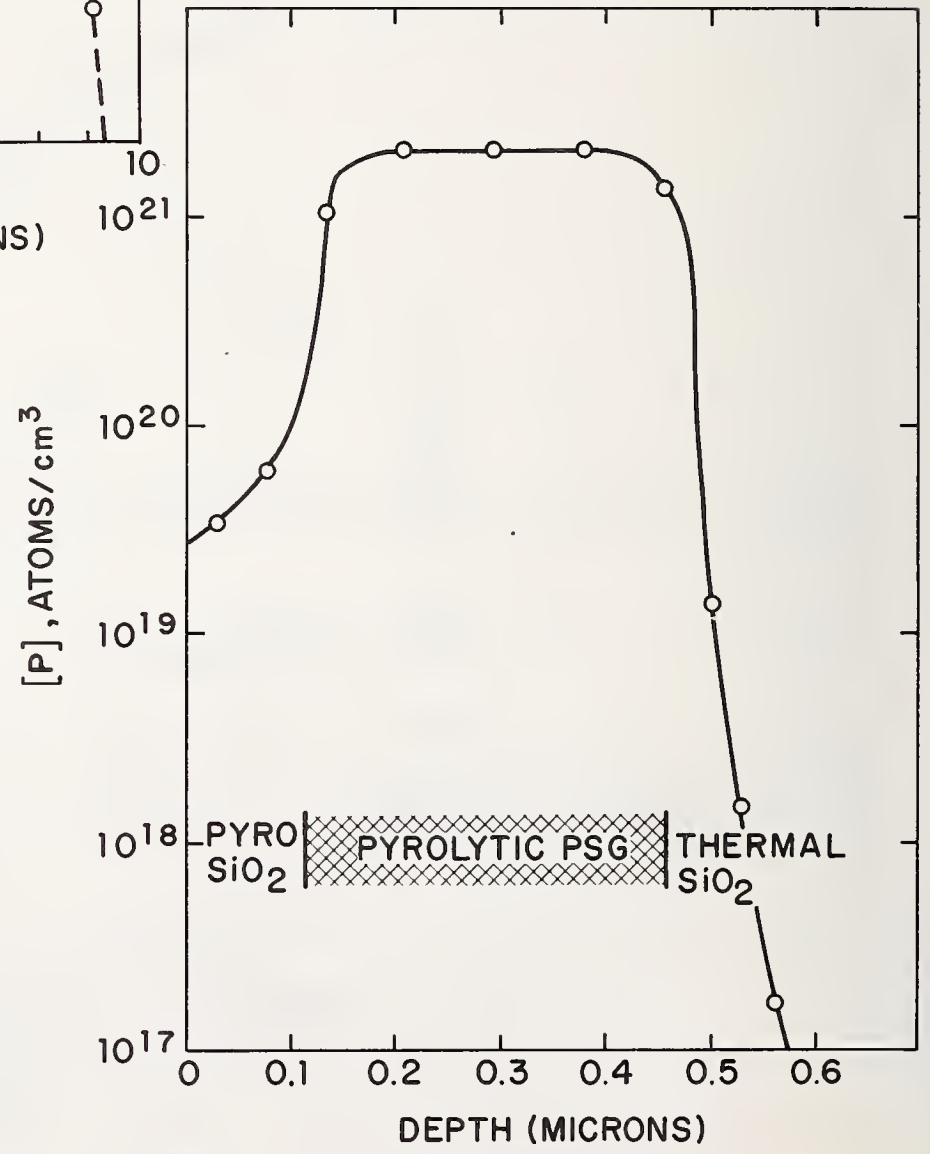
Fig. 3. Neutron activation profile of phosphorus impurity in multilayered SiO 2 film.
