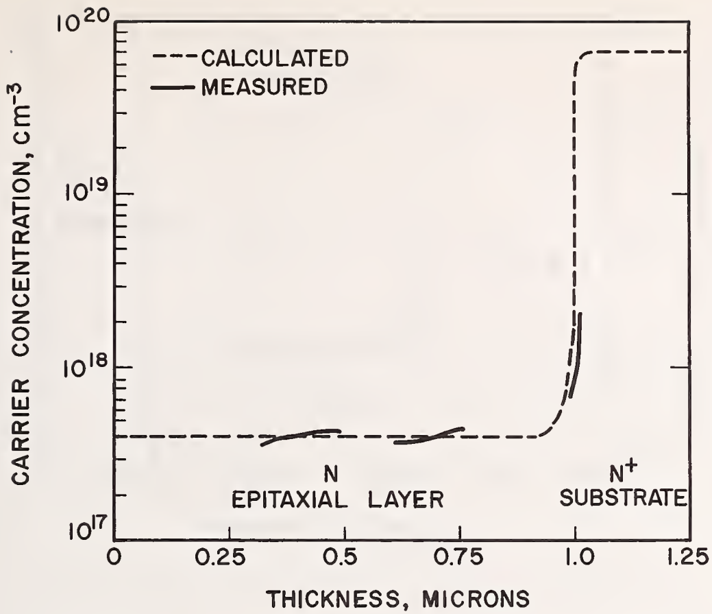
Fig. 4. Relationship of Epitaxial resistivity on Arsenic Concentration
