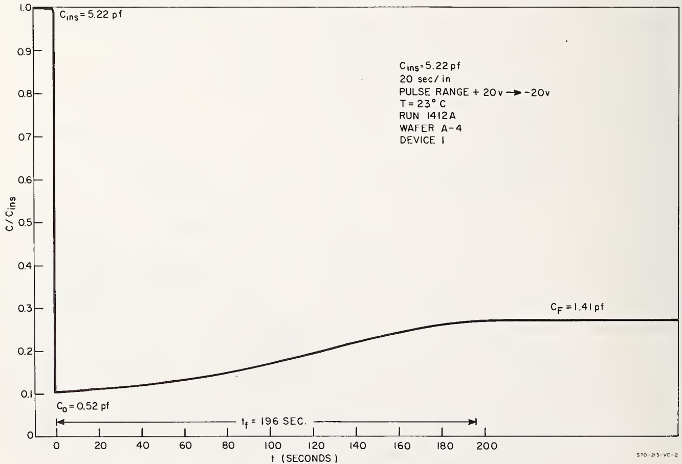
Fig. 10. Pulsed C-t Measurement of a MOS Structure
