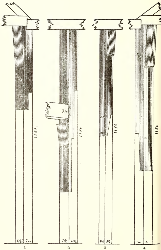
POSTS : WESTERN SIDE. Scale : 1 in. = 2 ft.
