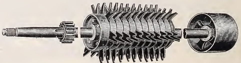
SMALLEY SHREDDER HEAD.
