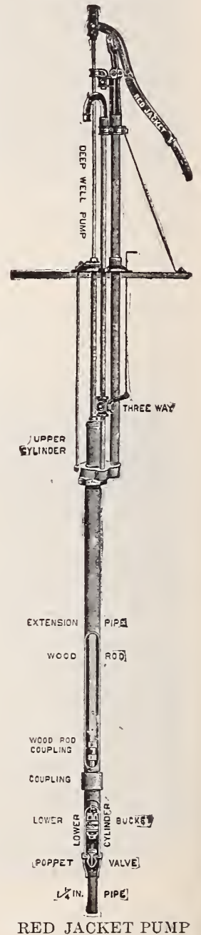
RED JACKET PUMP
