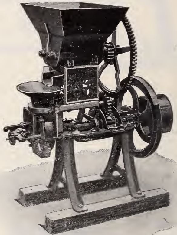
NO. 10 IDEAL DUPLEX MILL.
