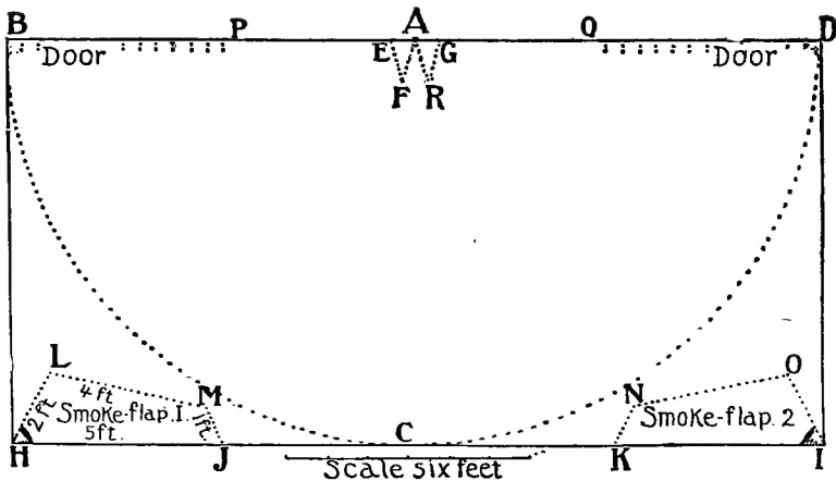
CUT I.—PATTERN FOR A SIMPLE 10-FOOT TEEPEE
