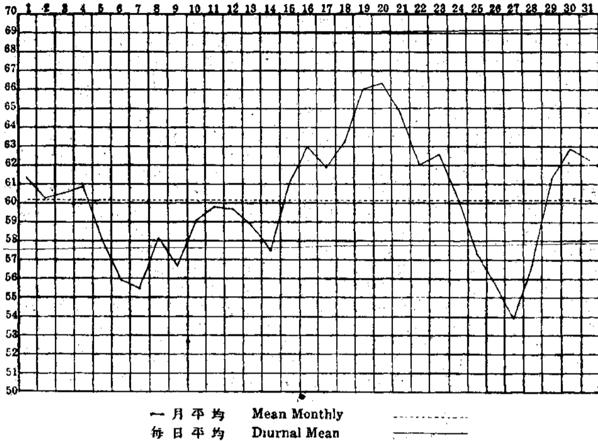
中華民國十七年十月份氣壓變遷圖 (700 mm +) The March of Barometric Pressure in the Month of October, 1928. (700 mm +) )
