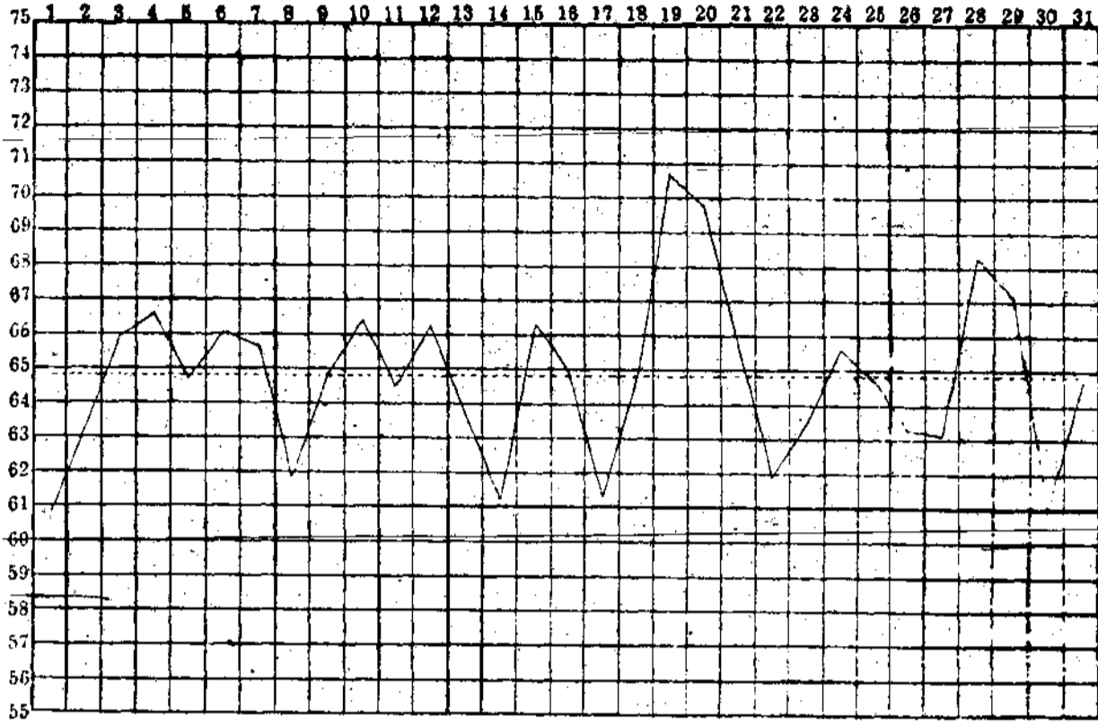
中華民國十七年十二月份氣壓變遷圖 (700 mm +) The March of Barometric Pressure in the Month of December, 1928. (700 mm +)
