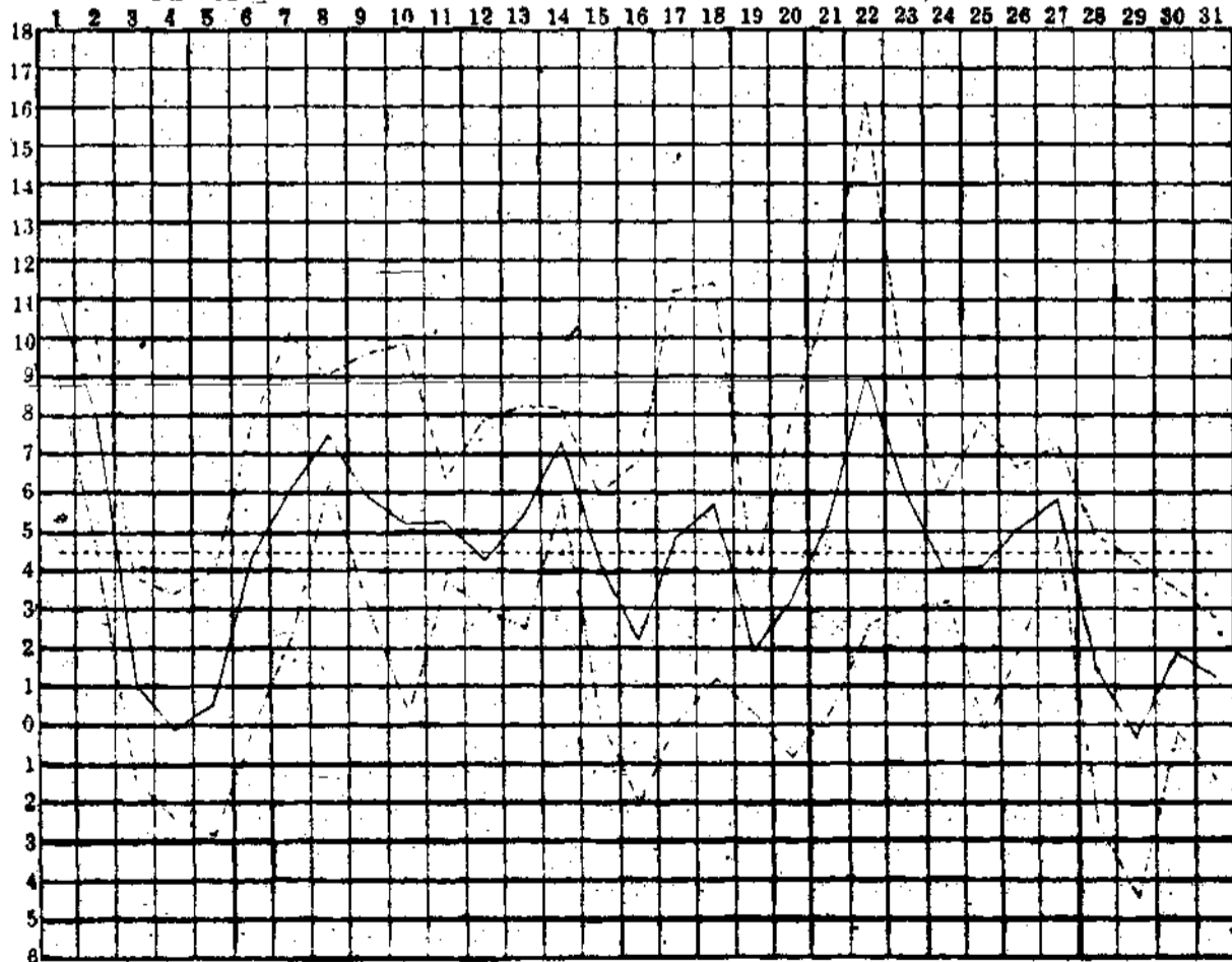
The March of Temperature in the Month of December, 1928. (°C)
