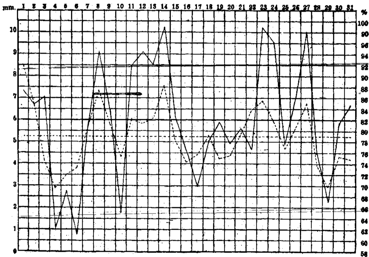
中華民國十七年十二月份濕度變遷圖 The March of Humidity in the Month of December, 1928.
