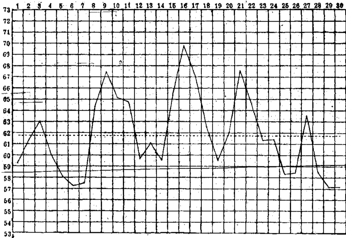
中華民國十七年十一月份氣壓變遷圖 (700 mm +) The March of Barometric Pressure in the Month of November, 1928 (700 mm +)
