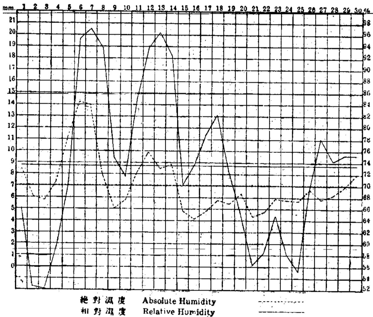
中華民國十七年十一月份濕度變遷圖 The March of the Humidity in the Month of November, 1928
