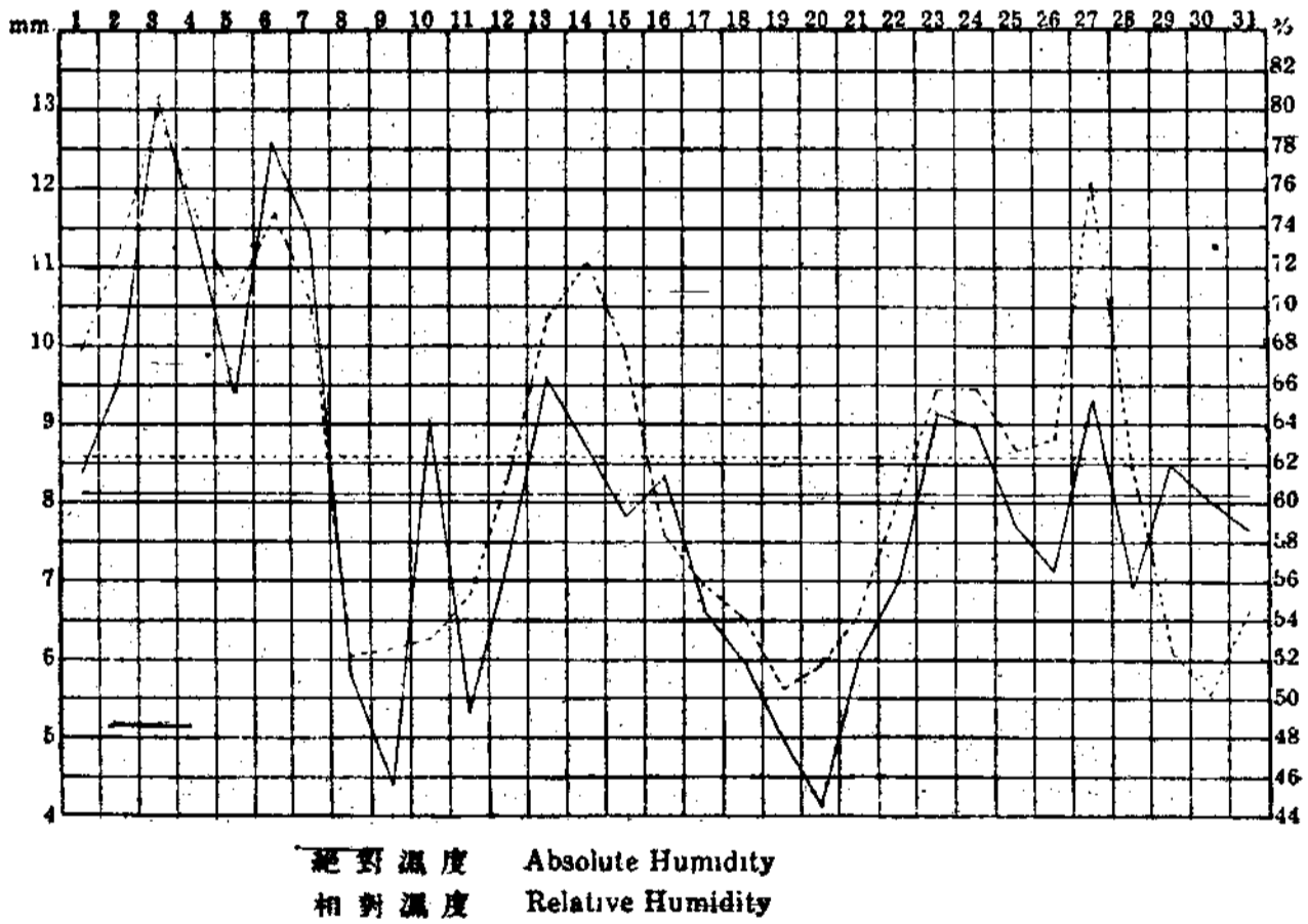
中華民國十七年十月份濕度變遷圖 The March of Humidity in the Month October, 1928.
