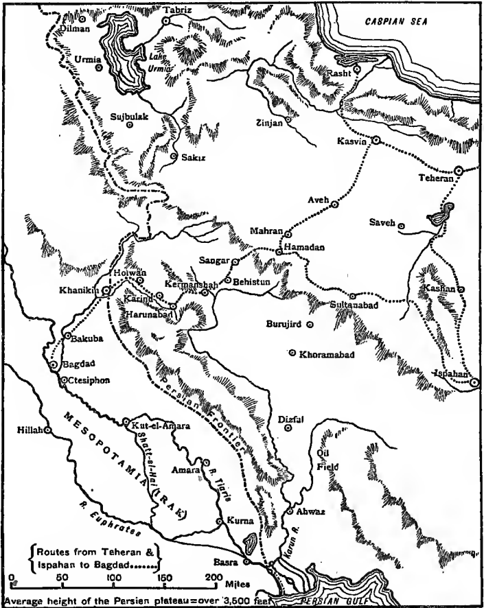
Scene of Baratov's Operations in Persia.
