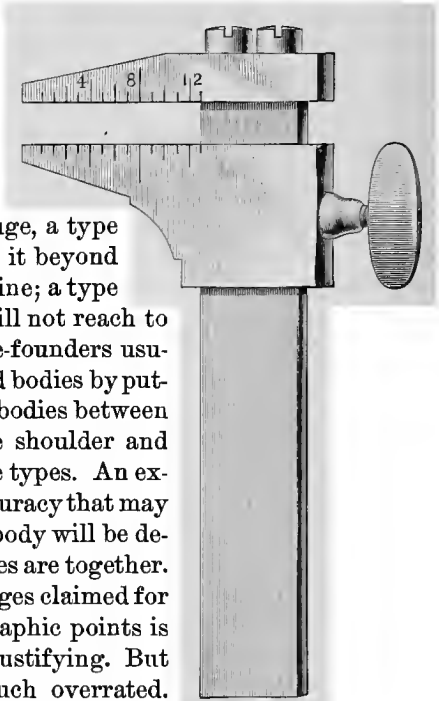
Type-gauge.
