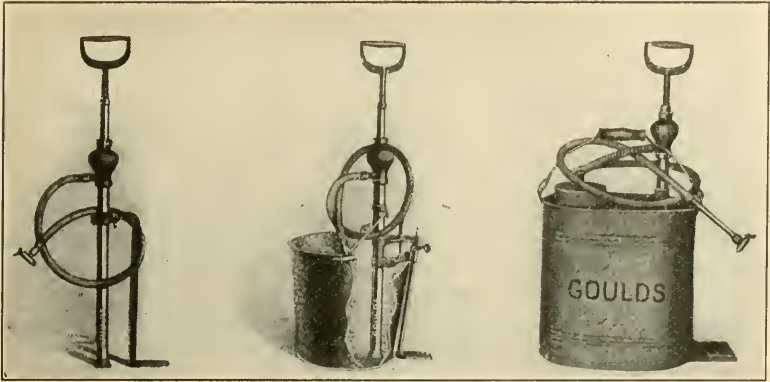
FIG. 238.—Spray pumps isolated and with bucket attachments.
