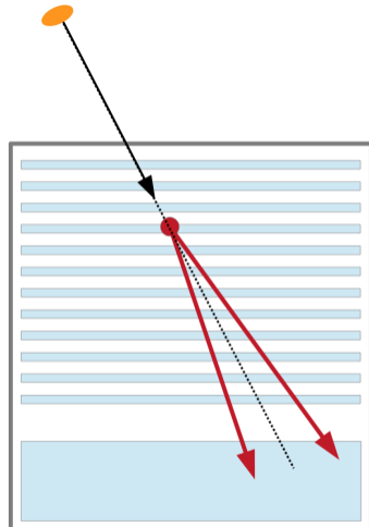
Pair event
