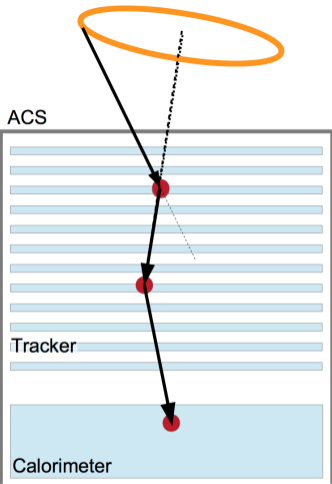
Compton event
