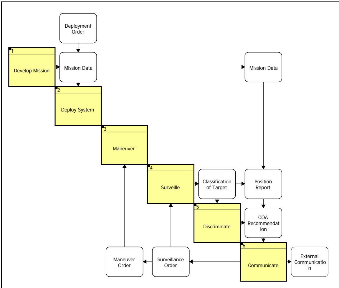
Figure 27. N2 matrix diagram for TUNAS sample UUV system (From: Brocht, Layne, Matson, McMurtrie, Schindler, & Vandenberg, 2009)
