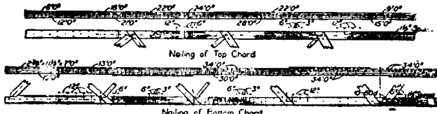
Details in Top and Bottom Chords.
