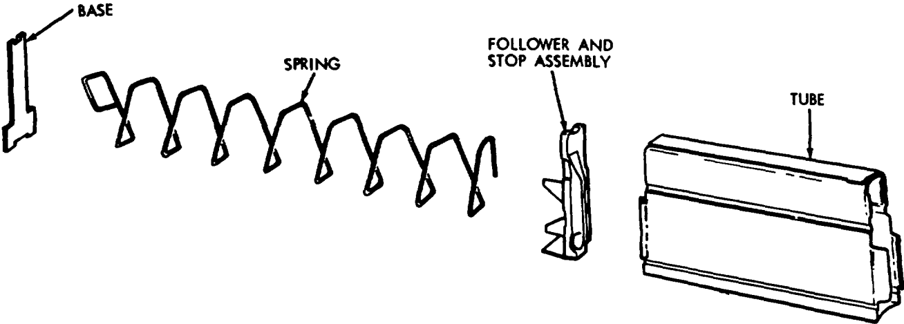
Figure 3-1. Magazine exploded view.
