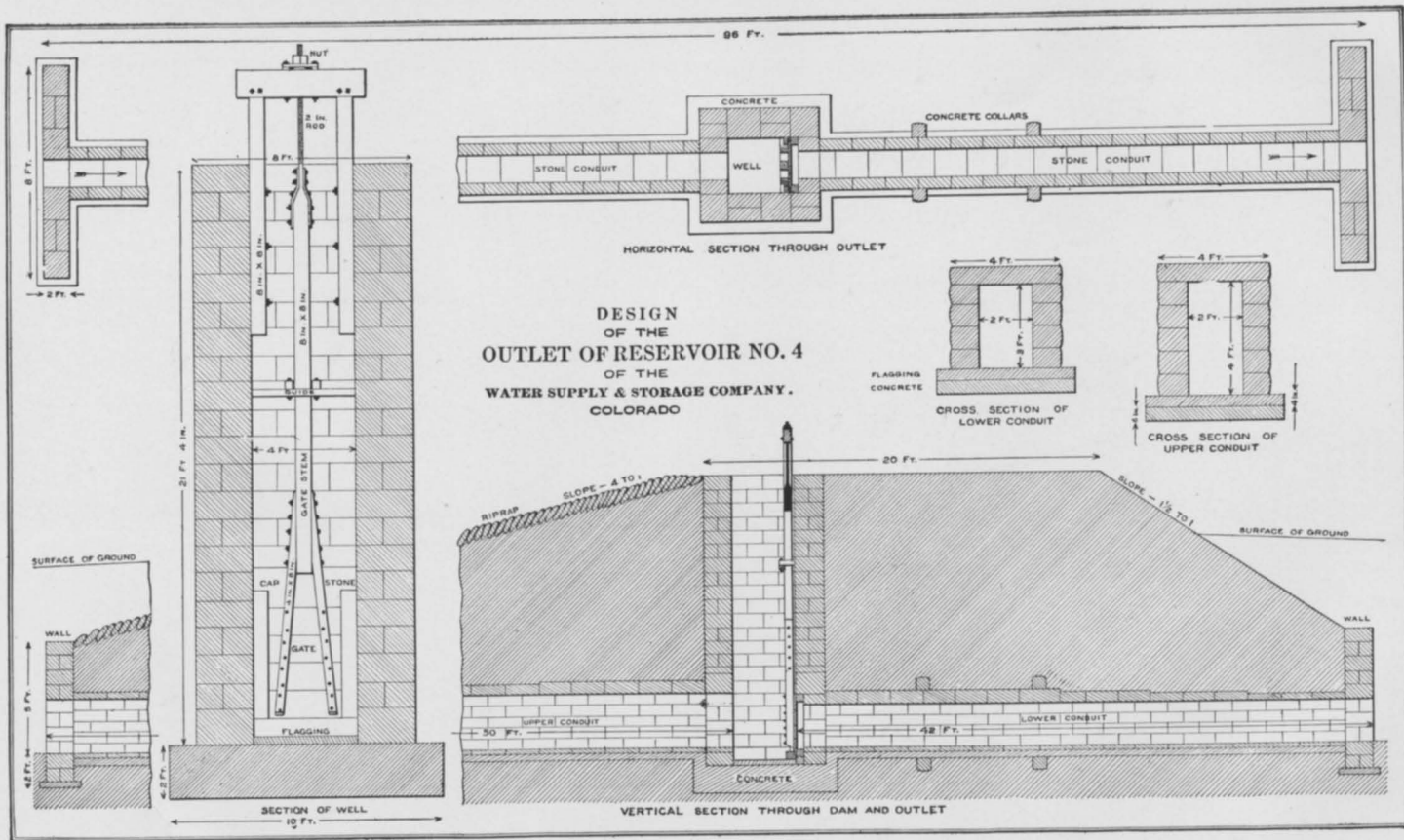
DETAILS OF CONSTRUCTION OF RESERVOIR DAM AND OUTLET.
