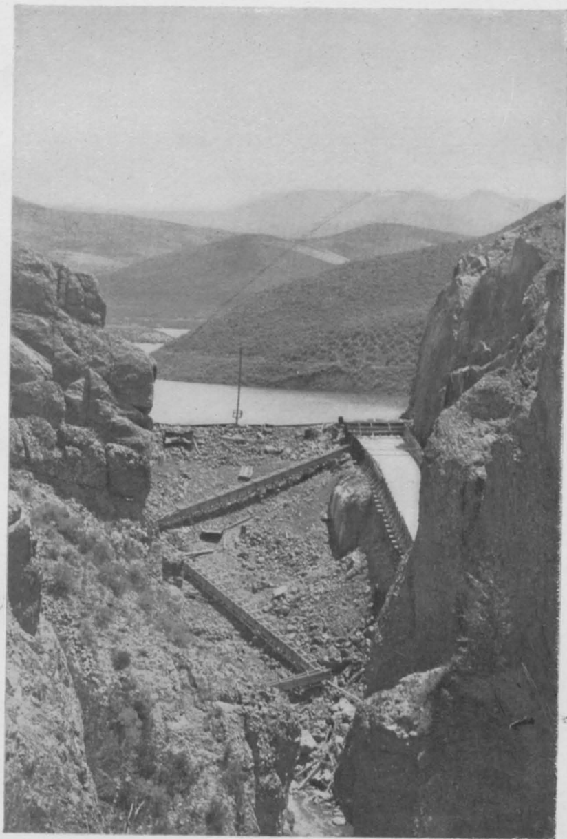
WASTEWAY, EAST CANYON CREEK RESERVOIR, UTAH.
