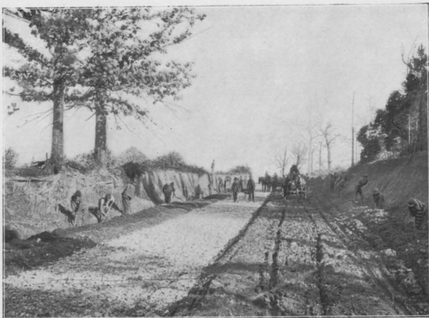
FIG. 1.—CONVICTS BUILDING A MACADAM ROAD IN MECKLENBURG COUNTY, N. C.
