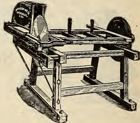
Appleton Slide Table Saw.
