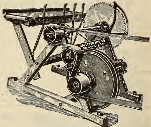
Appleton New Style Pole Saw.
