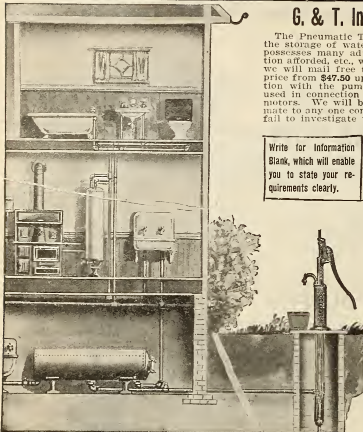
Invincible Horizontal Tank and Gould's Deep Well Pump.
