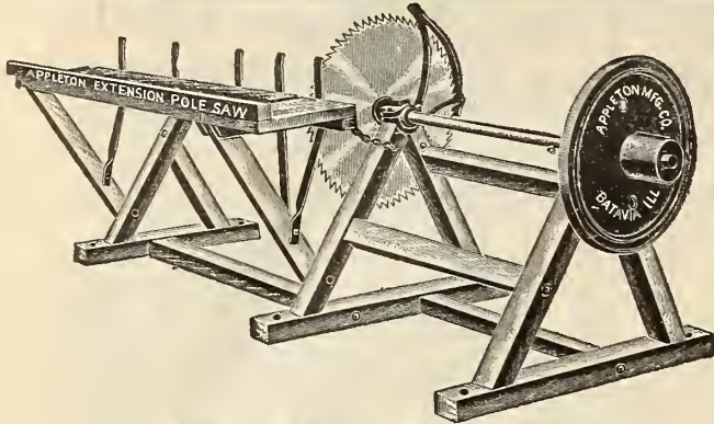
Appleton Extension Table Pole Saw.
