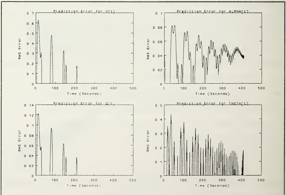
Figure 27: Prediction Error
