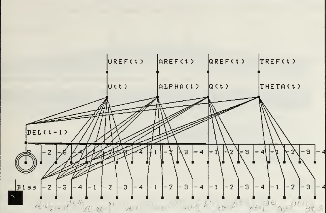
Figure 15: Neural Network Adaptive Controller Structure for A-4 Longitudinal Motion
