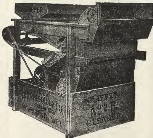
Clipper Cleaner No. 2-B
