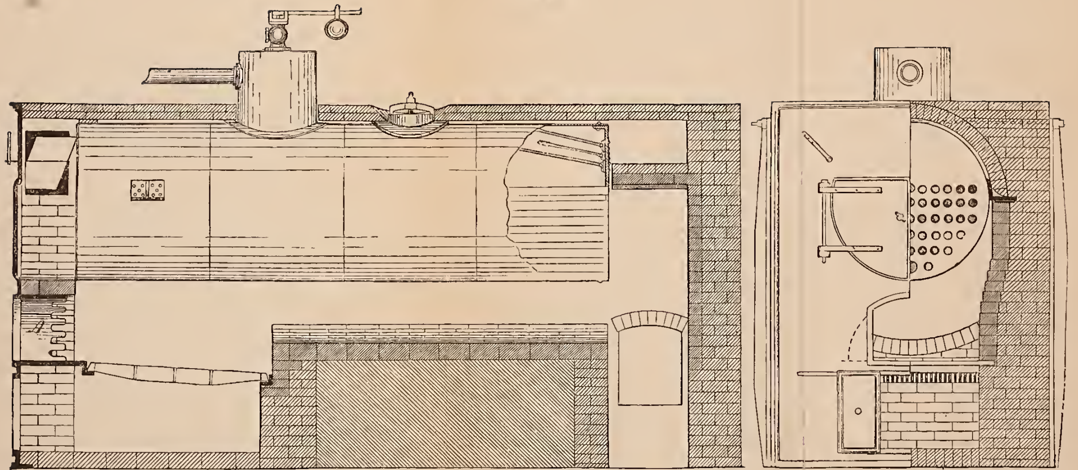
HORIZONTAL-MULTI-TUBULAR-BOILER.
