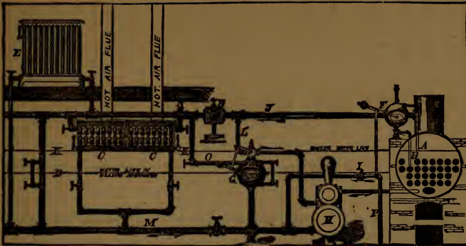
PATENT WATER-LINE SYSTEM.
