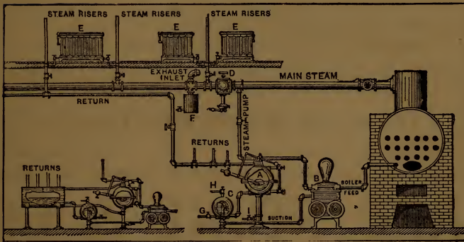
PATENT DRY-RETURN SYSTEM.
