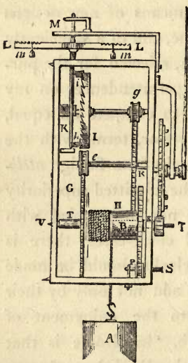
Old Balance-Clock.
