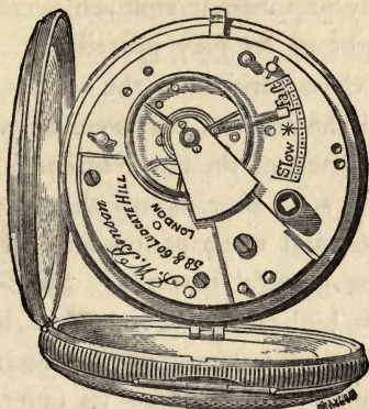
The Full Plate Patent English Lever.
