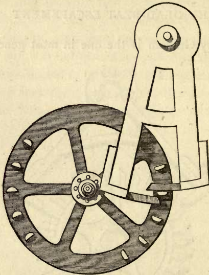
French Single-Pin Escapement.
