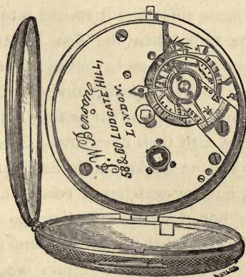
Three-Quarter Plate English Lever.
