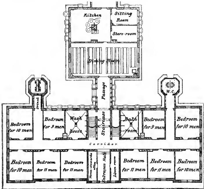
Ground Plan.
