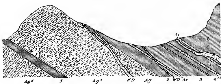
SECTION OF THE OAKELEY QUARRIES, FESTINIOG.*
