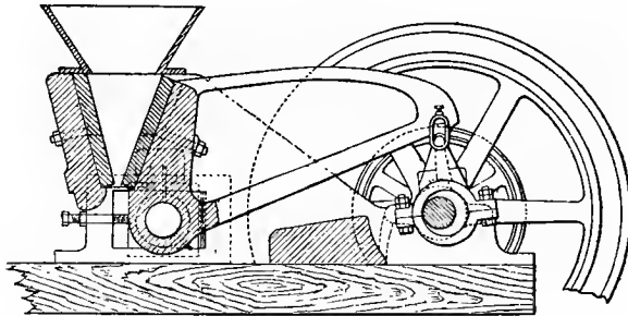
THE DODGE CRUSHER.
