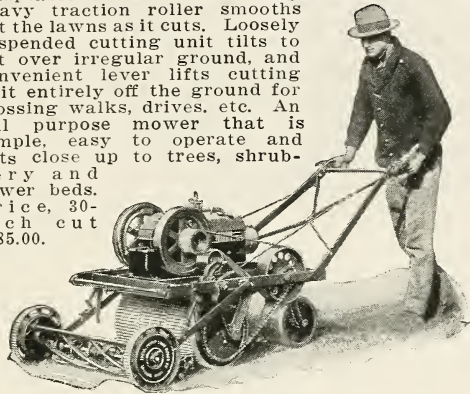
Ideal Mower Model 30.
