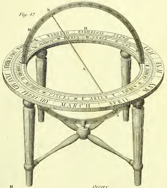
Orrery
