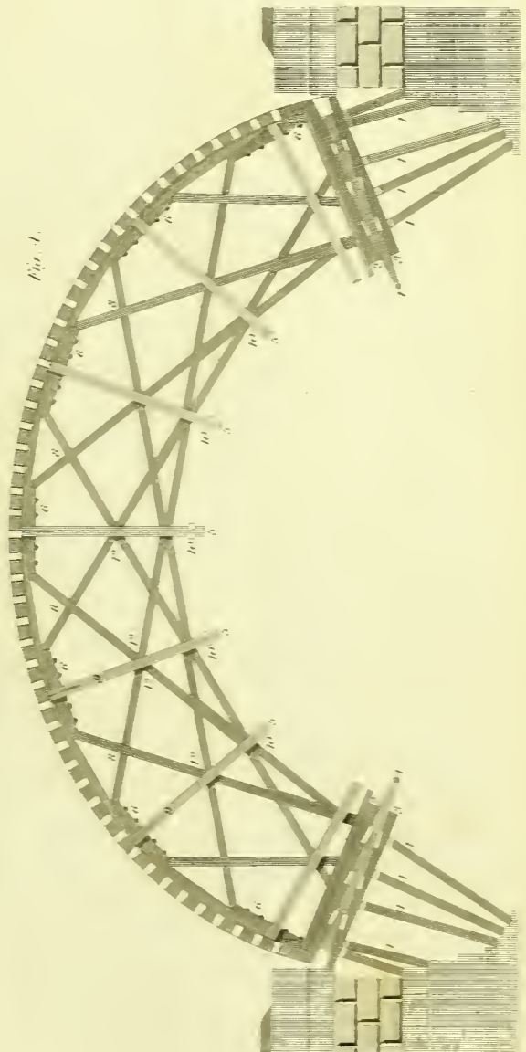
Centering for an Arch
