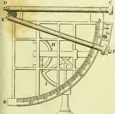
Astronomical Quadrant
