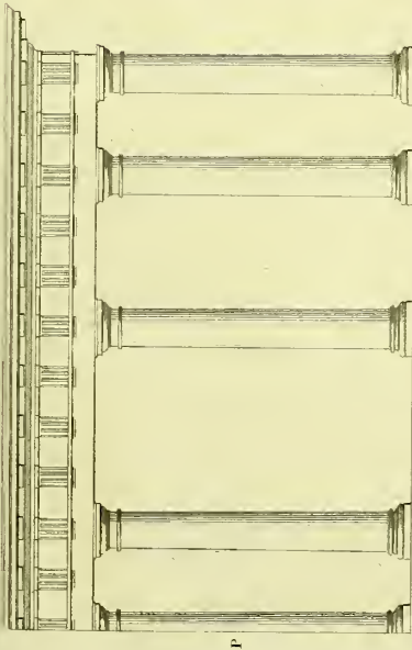
Doric Intercolumniation
