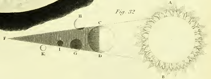
Lunar Eclipse
