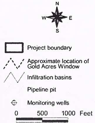
Figure 4.3.16 Infiltration Basin Location Map - Frome Area
