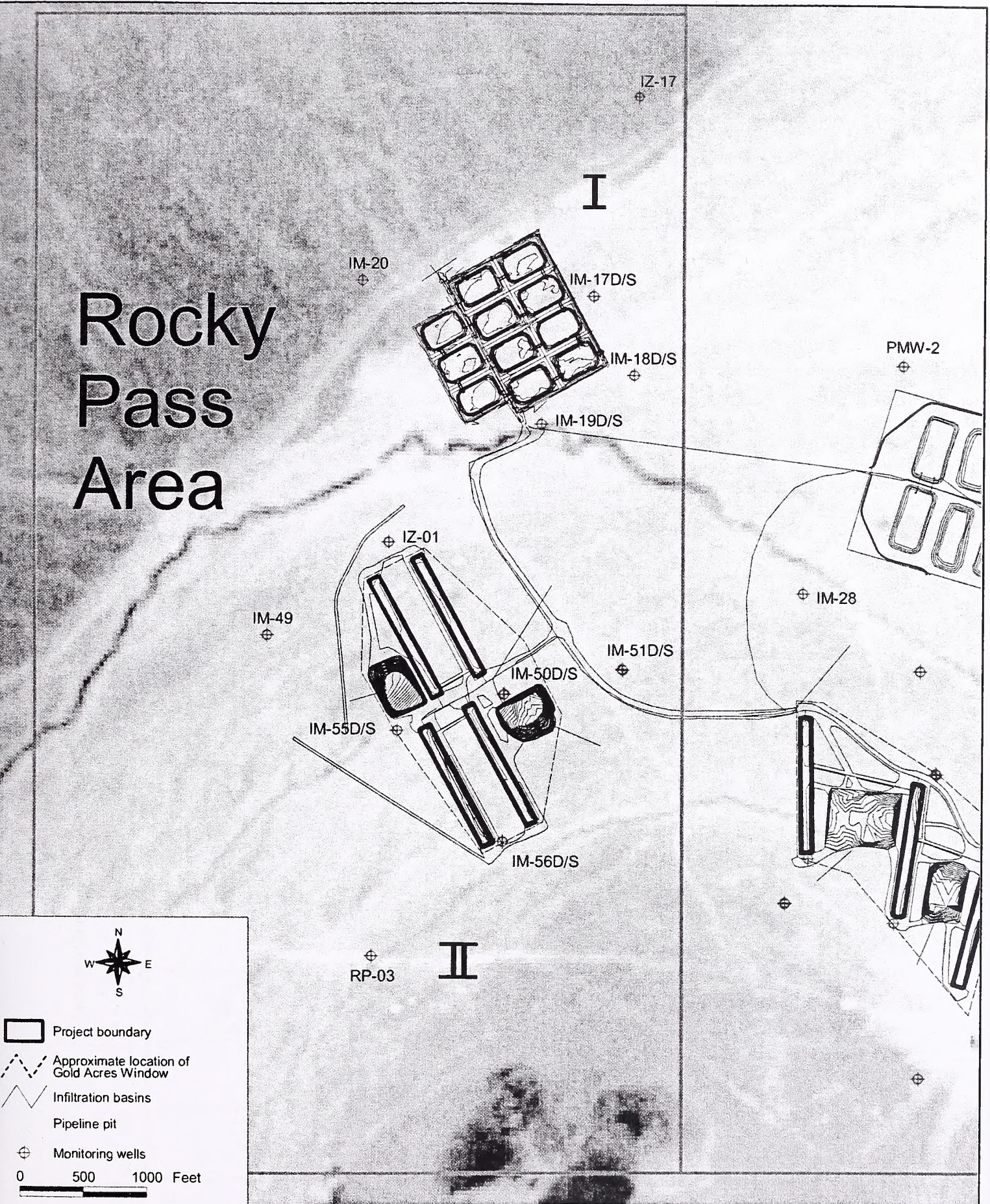
Figure 4.3.14 Infiltration Basin Location Map - Rocky Pass Area
