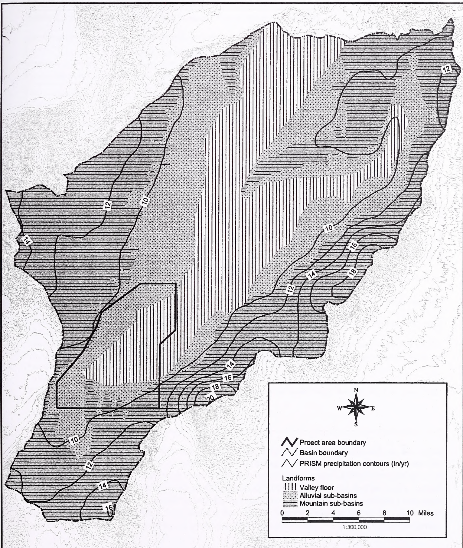
Figure 4.3.8 PRISM Precipitation Contours for Crescent Valley
