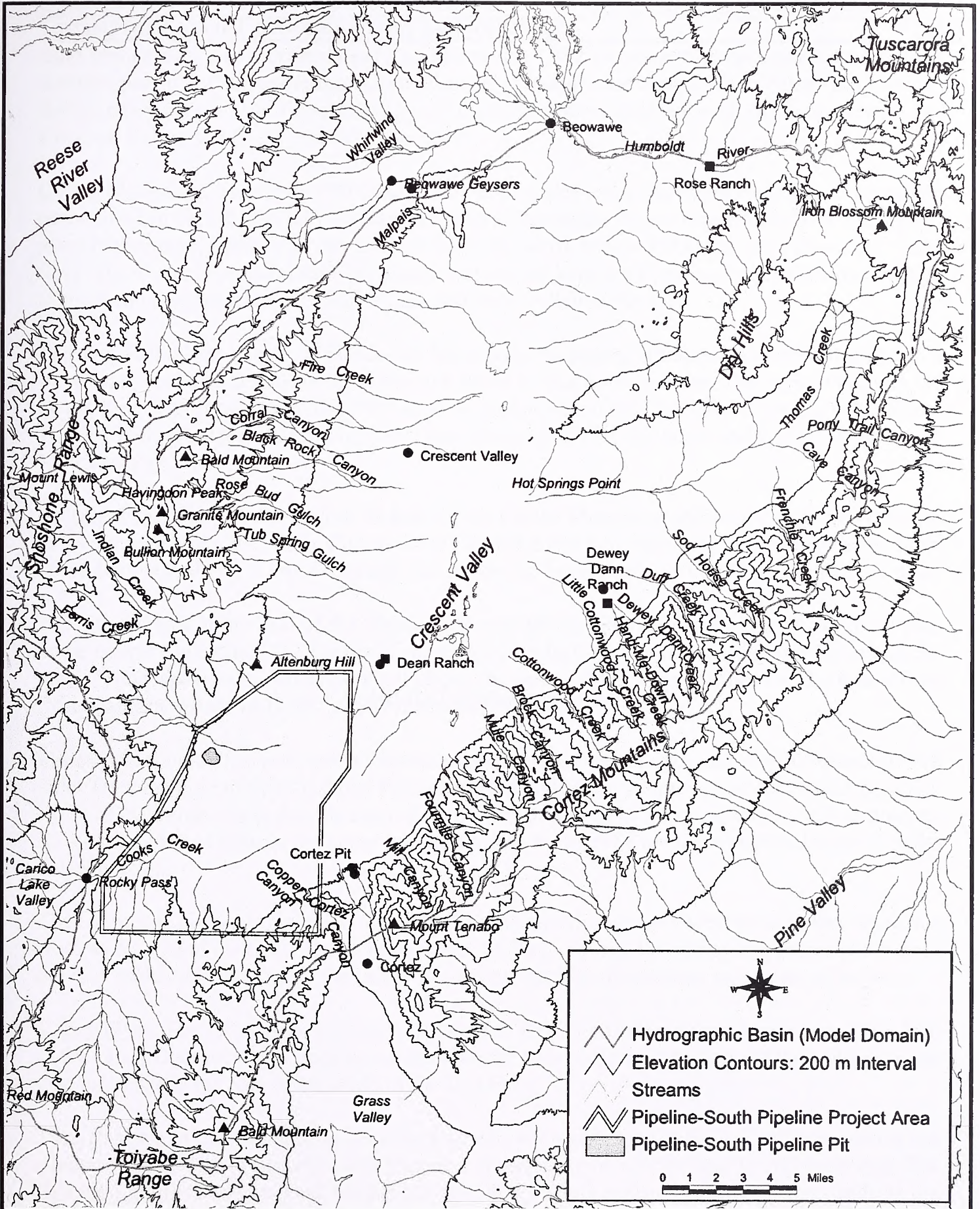
Figure 4.3.1 Physiographic and Hydrographic Features of Crescent Valley
