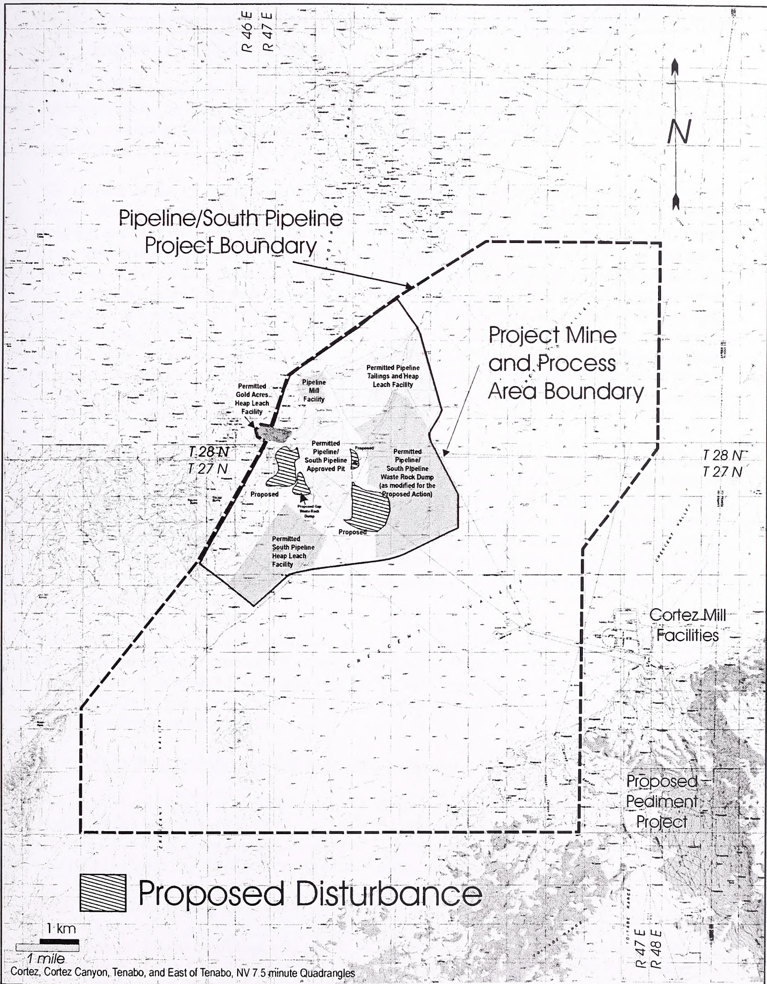
Figure 1.1.2 Project Area Map
