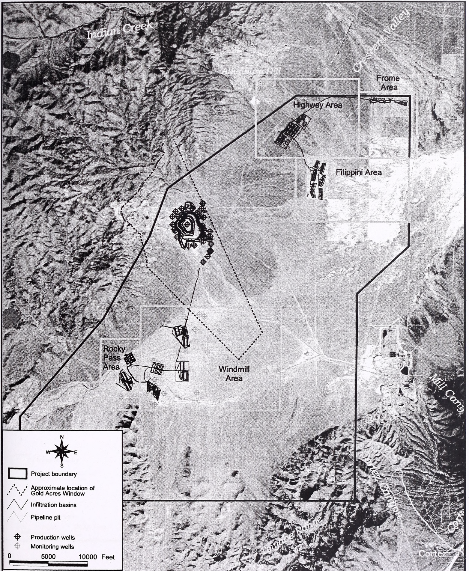
Figure 4.3.9 Infiltration Basin Location Map
