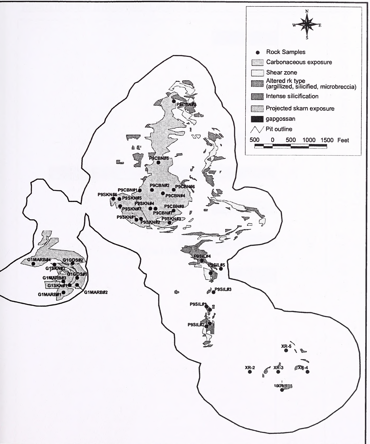
Figure 4.4.3 Location of Pipeline/South Pipeline Pit Expansion Rock Samples
