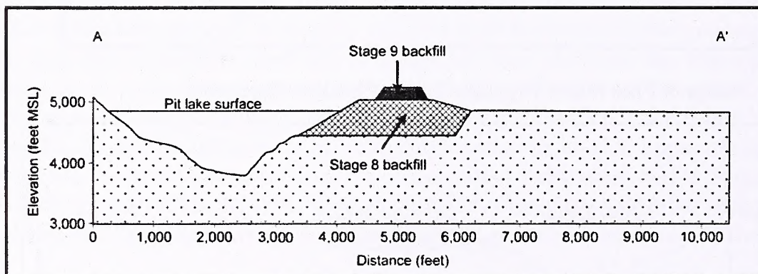
Figure 3.1.4: Stage 9 Cross Section A to A' through Pipeline/South Pipeline Open Pit
