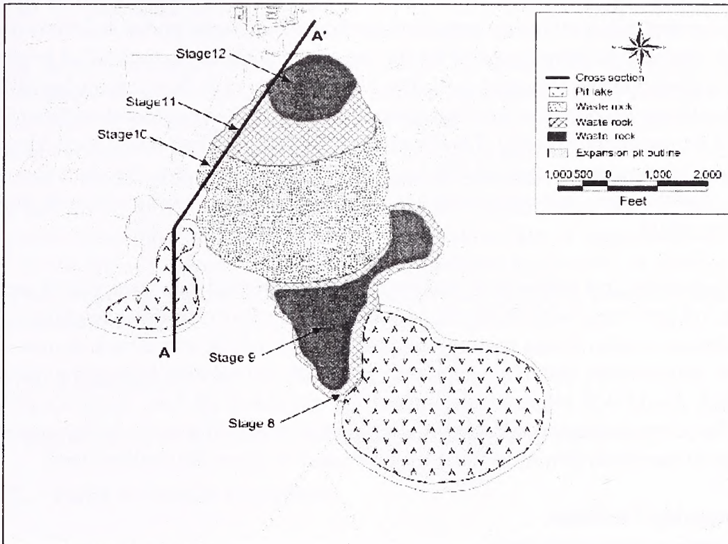
Figure 3.1.9: Stage 12 Plan View Pipeline/South Pipeline Backfilled Pit and the Gap Open Pit
