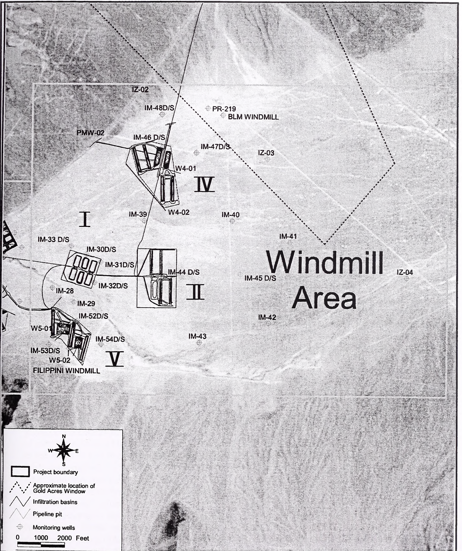
Figure 4.3.18 Infiltration Basin Location Map - Windmill Area
