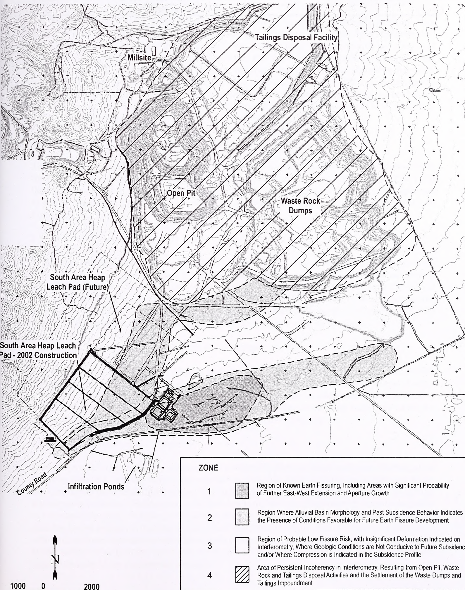
Figure 2.3.2 Preliminary Zoning of Earth Fissure Risk
