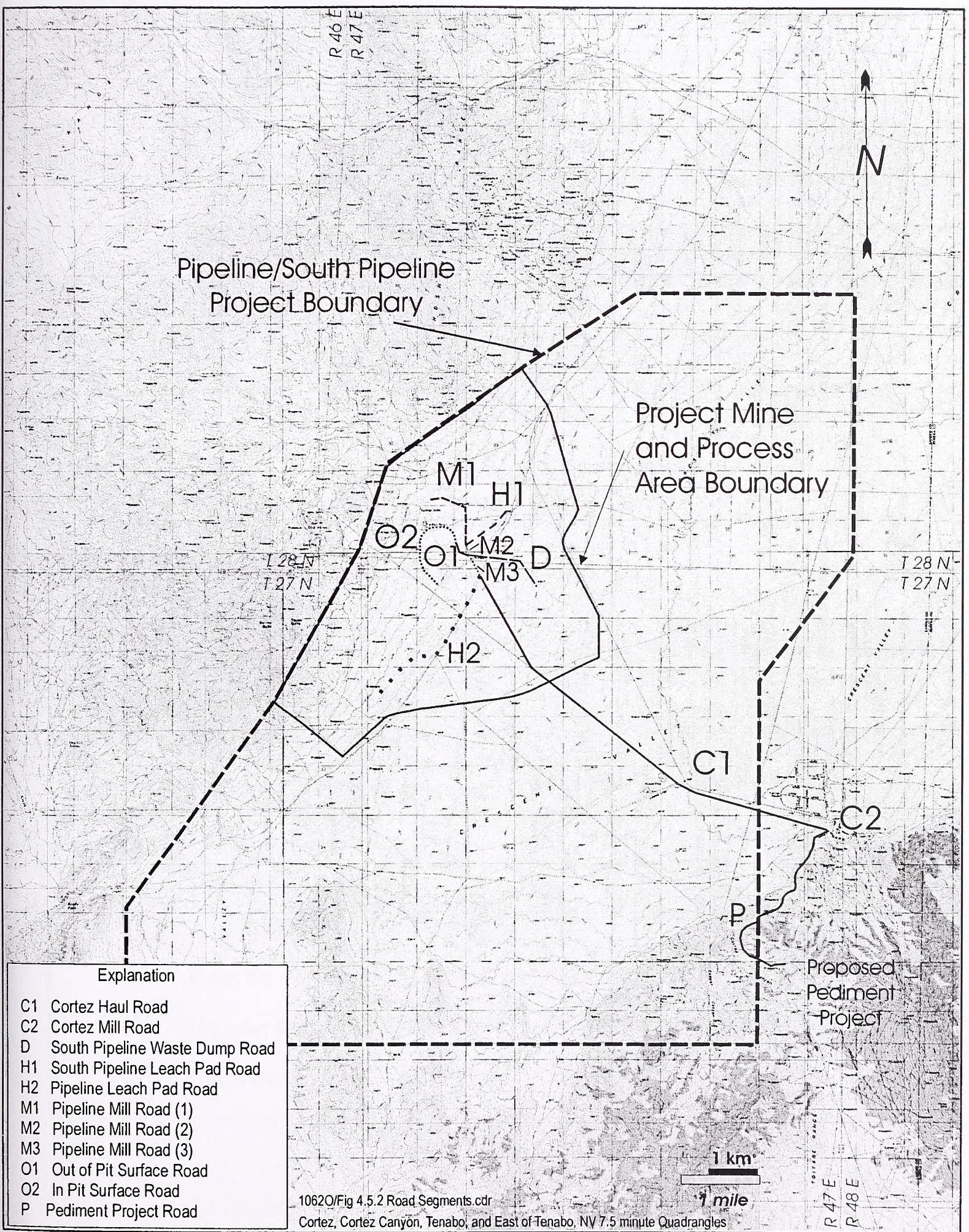
Figure 4.5.2 Road Segments Used to Model Fugitive Emissions
