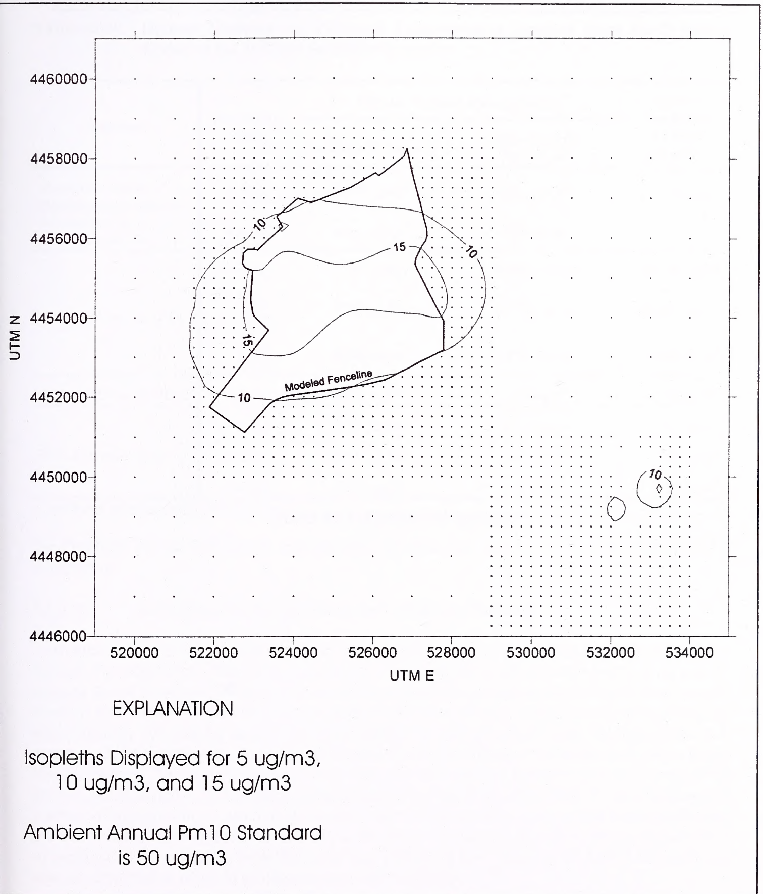
Figure 4.5.5 Isopleth of the Modeled Highest Annual PM10 Concentrations for the Proposed Action
