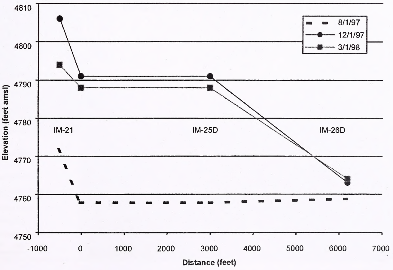
Figure 4.3.17 Water Levels at the Frome Infiltration Site
