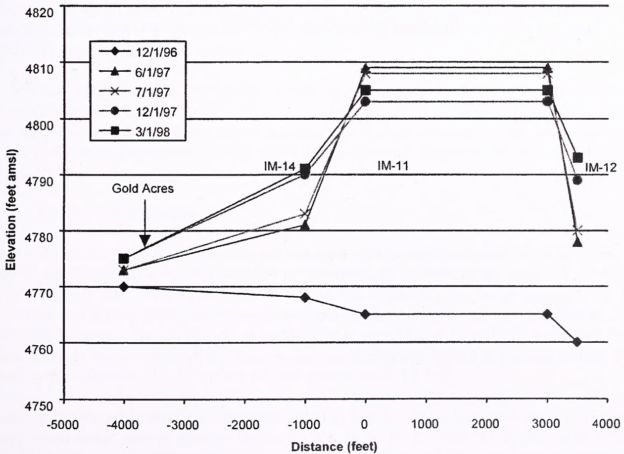
Figure 4.3.13 Water Levels at the Filippini Infiltration Site
