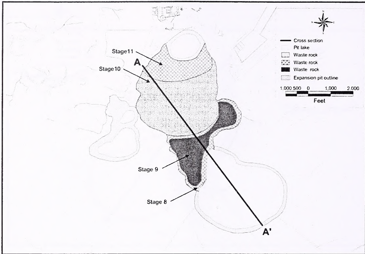
Figure 3.1.7: Stage 11 Plan View Pipeline/South Pipeline Open Pit
