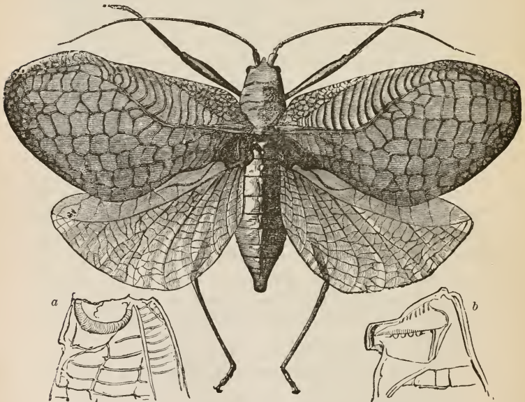
FIG. 12.— Chlorocœlus Tanana (from Bates). a. b. Lobes of opposite wing-covers.
