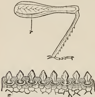
FIG. 13.—Hind-leg of Stenobothrus pratorum : r , the stridulating ridge; lower figure, the teeth, forming the ridge, much magnified (from Landois).
