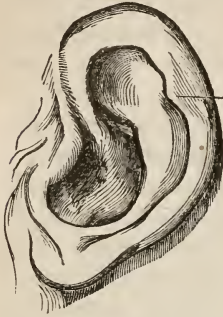
FIG. 2.—Human Ear, modelled and drawn by Mr. Woolner. a. The projecting point.
