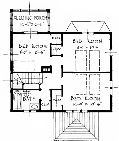
The Second-floor Plan
