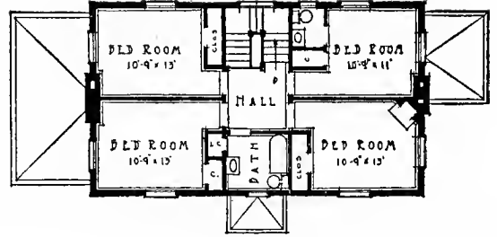
The Second-Floor Plan
