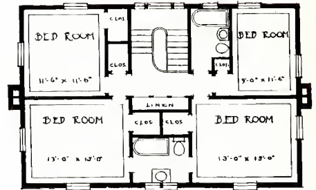
The Second-floor Plan
