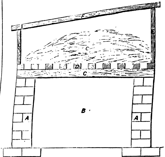
FIG. 563. SECTIONAL END VIEW OF A CHAMBERED FRAME.
