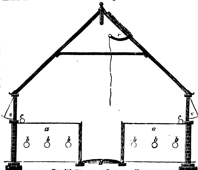
FIG. 560. SECTION OF SPAN-ROOF HOUSE a a, Space for Bottom Heat; b b b b b, Hot-water Pipes; c c, Pipes for Top Heat; d, Path; e e, Ventilators.
