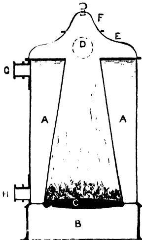
FIG. 260. VERTICAL SECTION OF CYLINDER BOILER.
