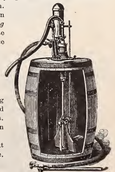
PEERLESS BARREL SPRAYER.
