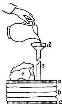
a , boards. b , leather. c , bamboo. d , tin funnel. e , rock or weight.
