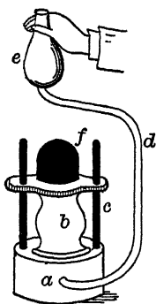
a , wood. b , e , leather. c , brass rods. d , rubber tube. f , bowlder or weight.
