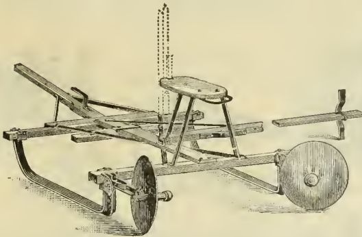
As a Furrower.
