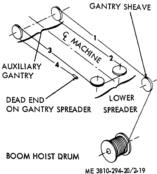
Figure 2-19. Backhoe auxiliary gantry suspension reeving.
