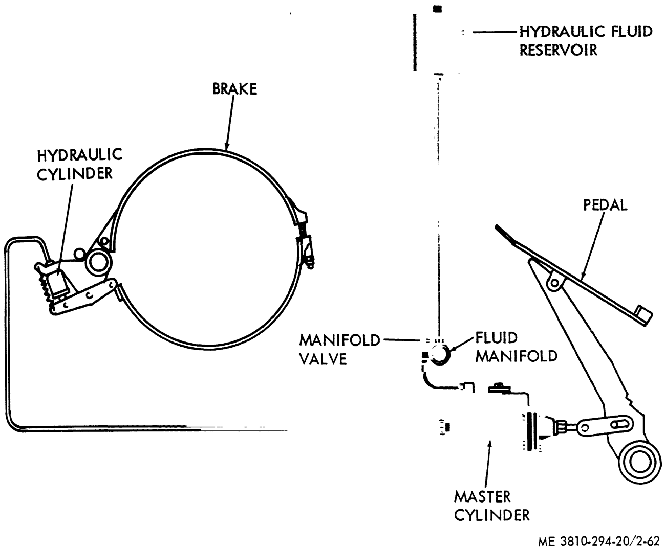
Figure 2-62. Hydraulic system, schematic diagram.
