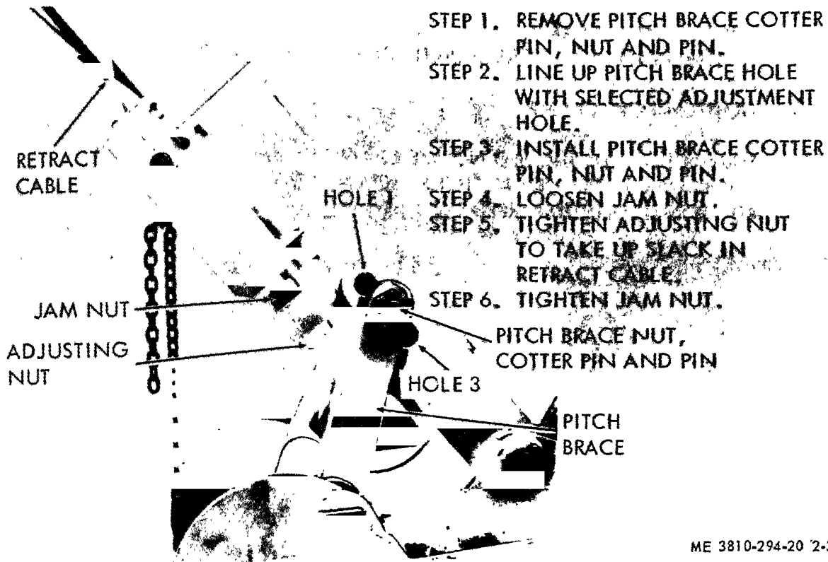
Figure 2-33. Rake angle and retract cable adjustment.
