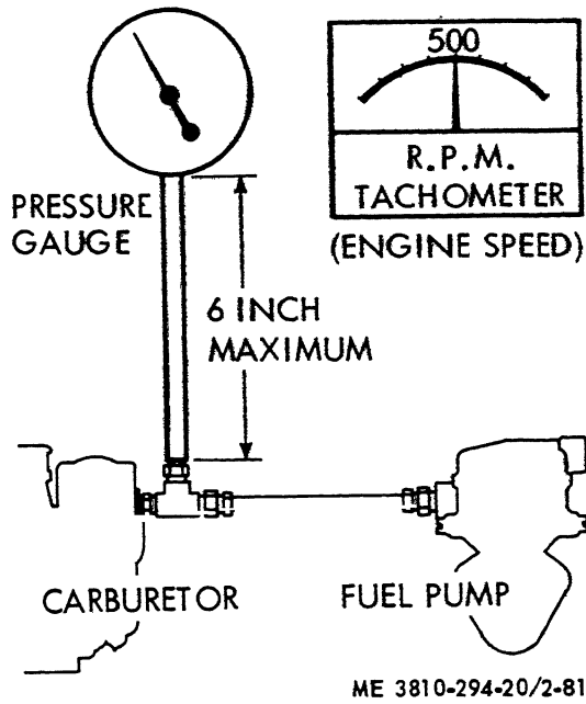
Figure 2-81. Checking fuel pump output pressure.
