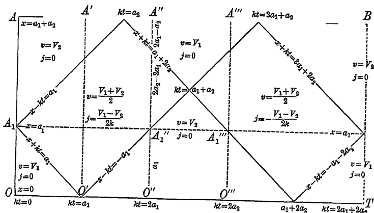
CASE a_1 < a_2 < 2a_1 .
