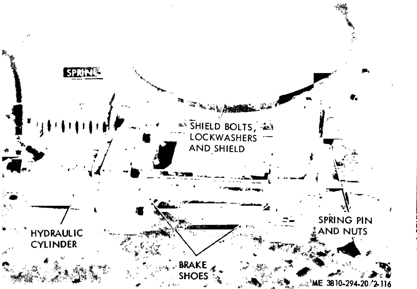
Figure 2-116. Swing brake shoes removal and replacement.
