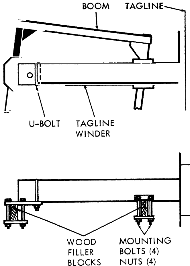
Figure 2-12. Tagline winder installation.
