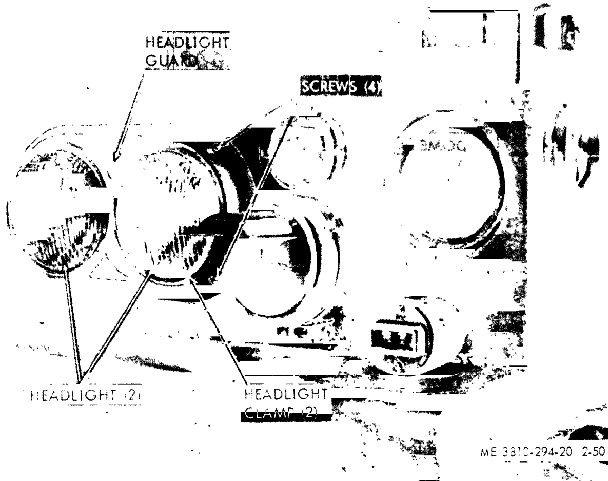
Figure 2-50. Headlights, replacement.
