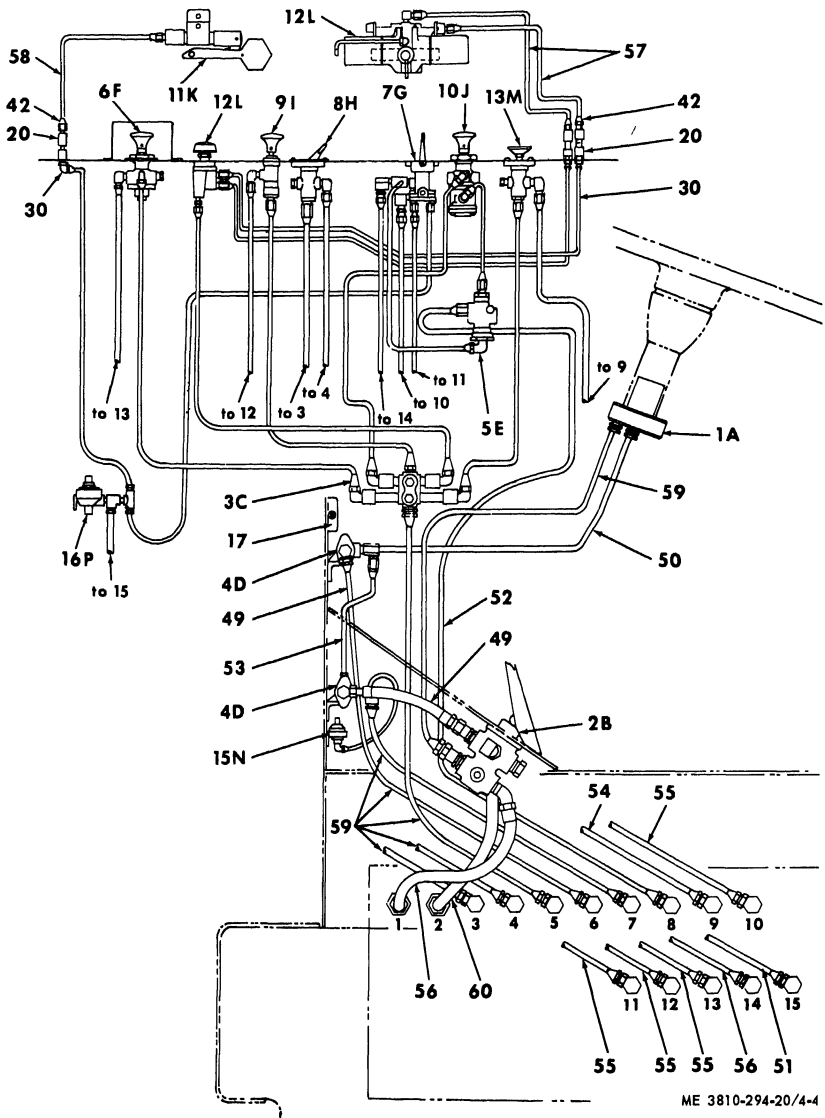
Figure 4-48. Air brake system piping diagram, valves, hoses, and fittings, removal and replacement (Sheets 1 through 3)
