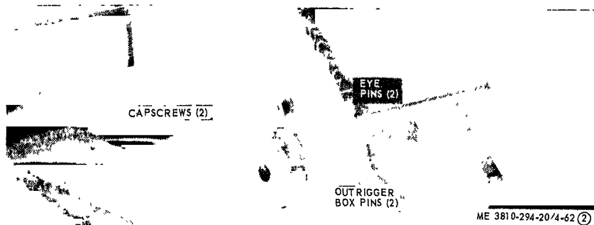
Figure 4-62. Outrigger, removal and replacement (sheet 2 of 2).
