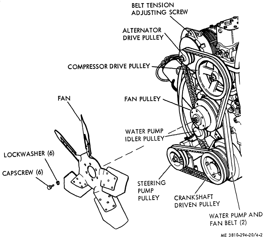
Figure 4-22. Engine belt and pulley arrangement, removal and replacement.
