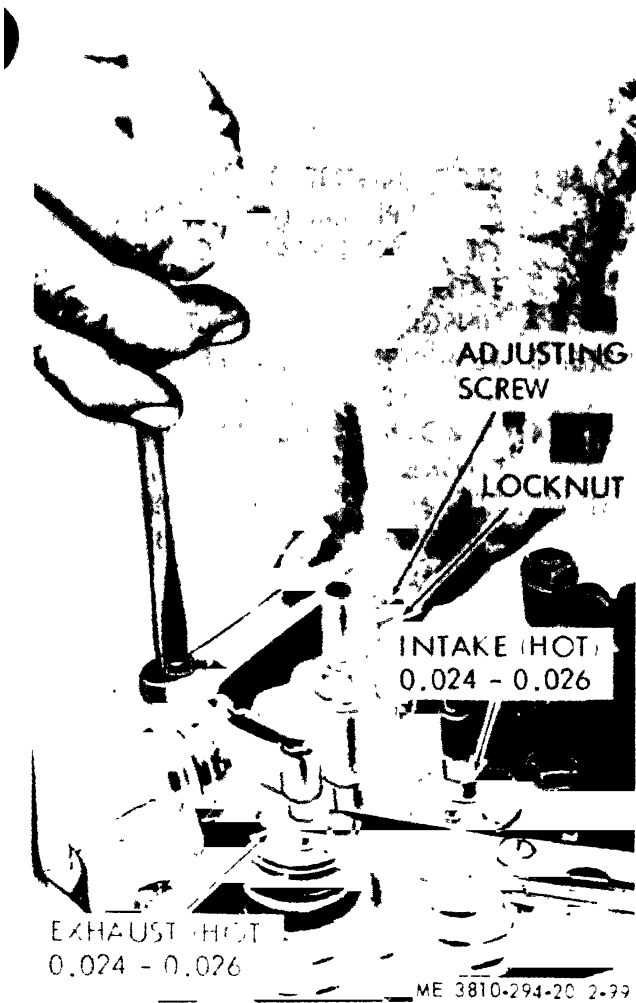
Figure 2-99. Adjusting valve stem to rocker arm clearance.
