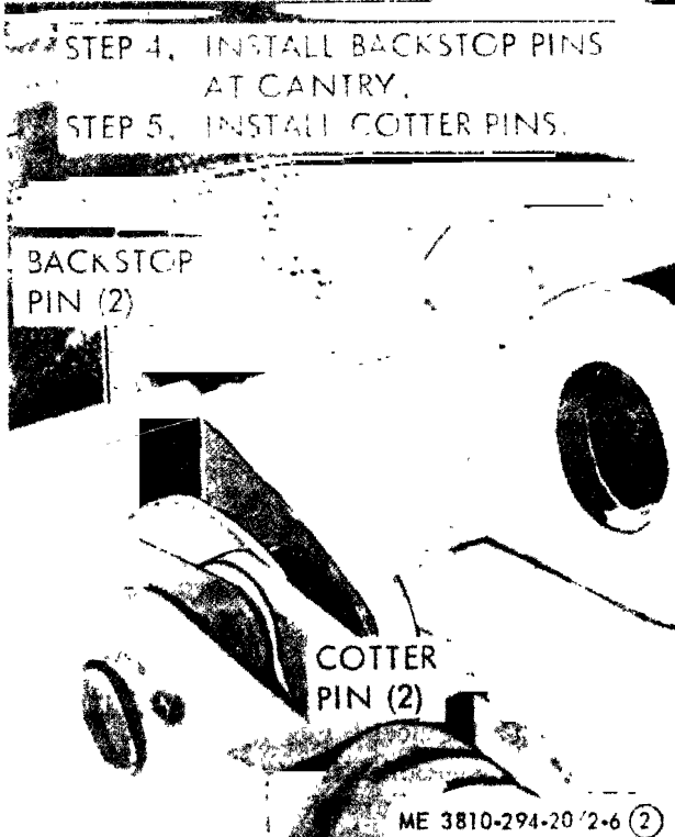
Figure 2-6. Boom backstop installation. (Sheet 2 of 2)
