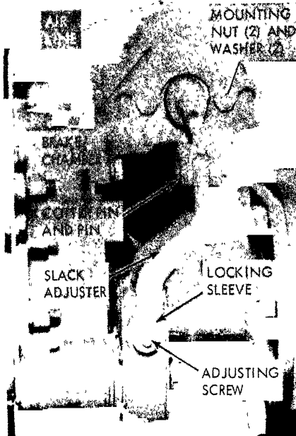
Figure 4-49. Front wheel brake chamber, removal and replacement.
