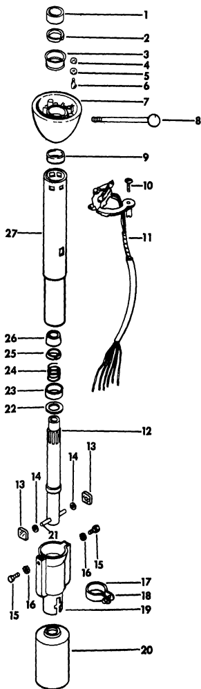
Figure 4-47. Steering column, exploded view.
