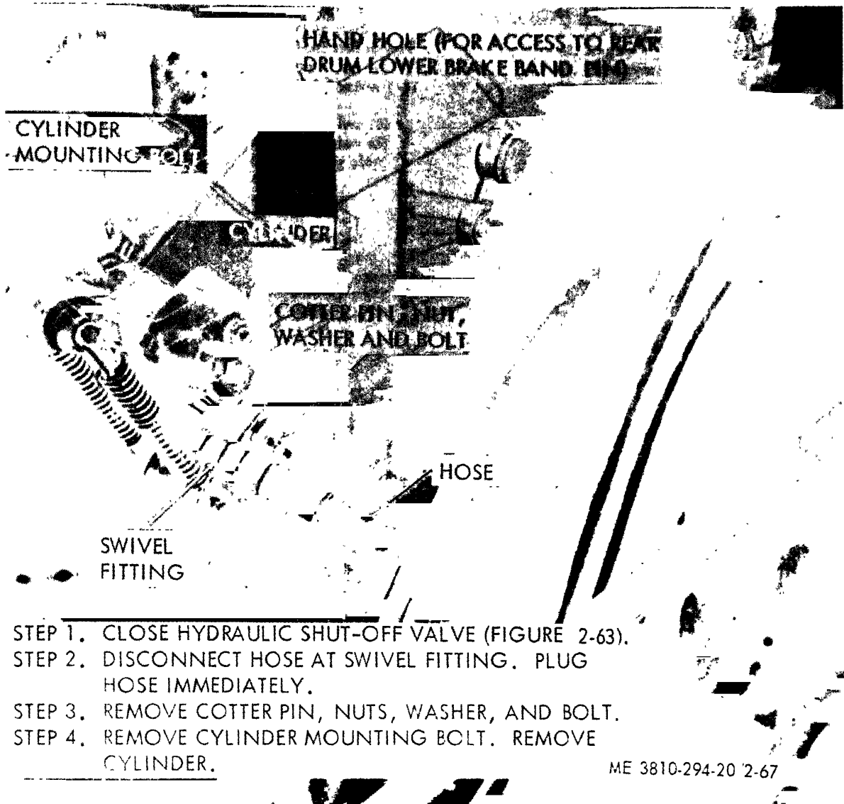
Figure 2-67. Hydraulic cylinders, replacement.
