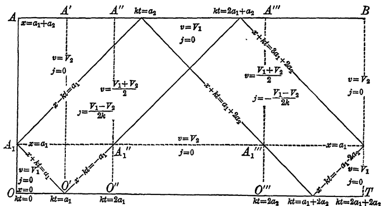
CASE 2a_1 < a_2 .
