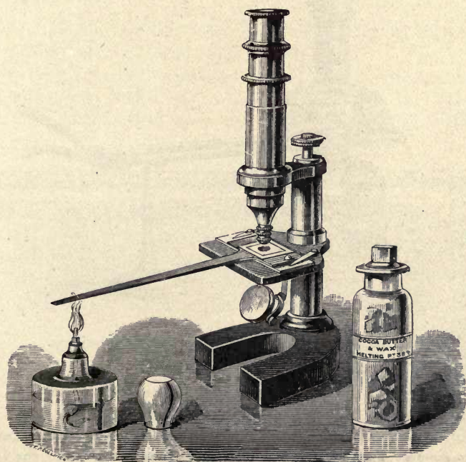
FIG. 51.—WARM STAGE SHOWN IN OPERATION.
