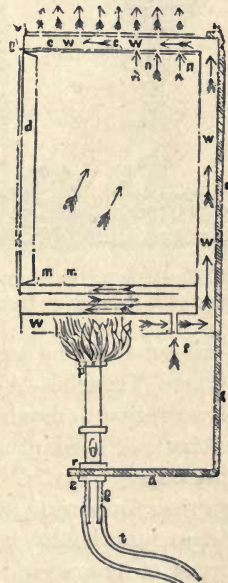
FIG. 252.—SECTION OF HOT-AIR STERILISER.
