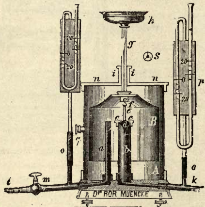
FIG. 269.—MOITESSIER'S GAS-PRESSURE REGULATOR.
