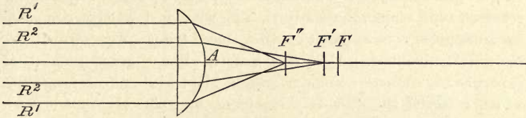
FIG. 12.—SPHERICAL ABERRATION.
