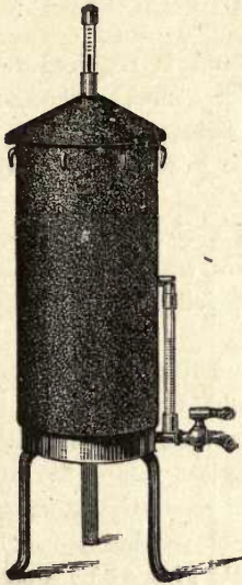
FIG. 250.—Koch's STEAM-STERILISER.
