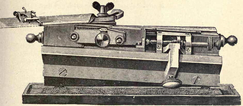
FIG. 28.—JUNG'S MICROTOME.
