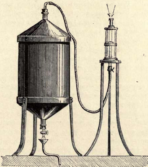
FIG. 73.—POUCHET'S AEROSCOPE.
