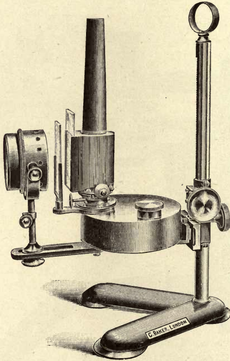
FIG. 21.—MICROSCOPE LAMP.
