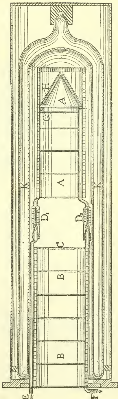
FIG. 3.—STANDARD WATER-FLOW PYRHELIOMETER.
