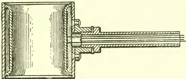
FIG. 2.—BULB OF MICRO-THERMOMETER.
