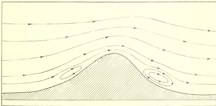
FIG. 2.—WIND EDDIES.
