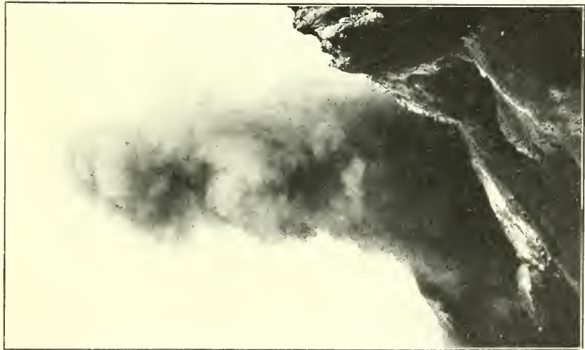
FIG. 1.—"STROMBOLIAN" EXPLOSION, 1912.
