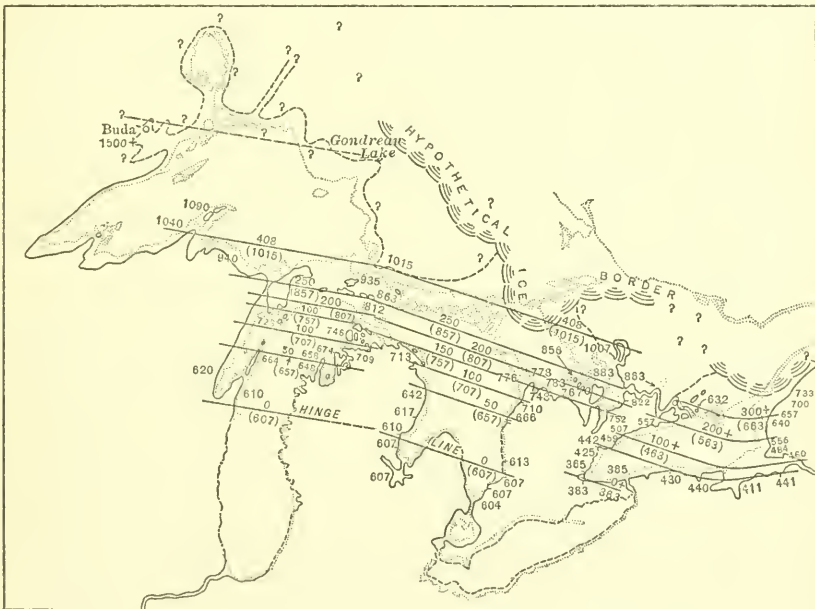
FIG. 7.—ISOBASES OF LAKE ALGONQUIN.
