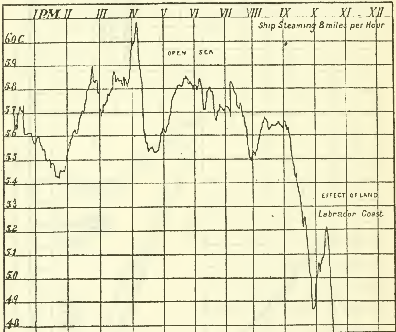
FIG. 4.—MARINE MICRO-THERMOGRAM, SHOWING EFFECT OF LAND.
