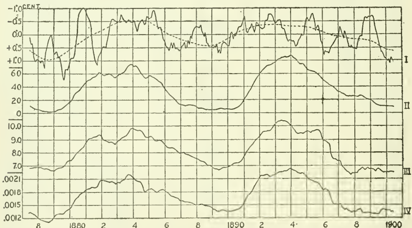
FIG. 7.—SUN-SPOTS AND THE EARTH'S TEMPERATURE AND MAGNETISM.
