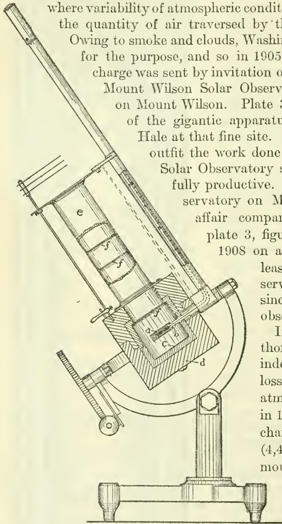
FIG. 4.—THE SILVER-DISK PYRHELIOMETER.
